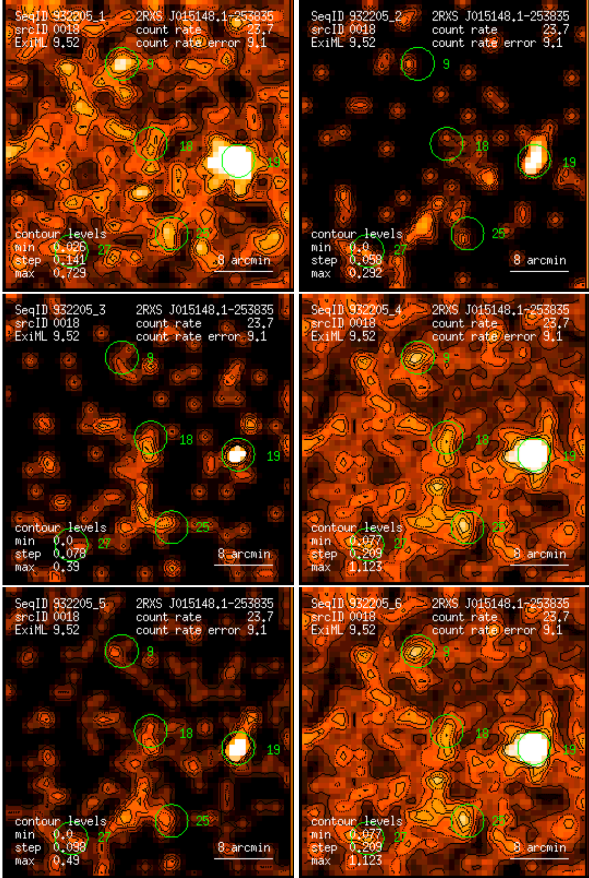
Figure 18: RASS 932205: detection 0018: band rate images, Gaussian filter: (1) PSPC channels 11 – 41, (2) 52 – 90, (3) 91 – 201, (4) 11 – 235, (5) 52 – 201, (6) 11 – 201. Broad band rates in counts/ks. Band rate contour levels in counts/ks/arcmin 2 .
