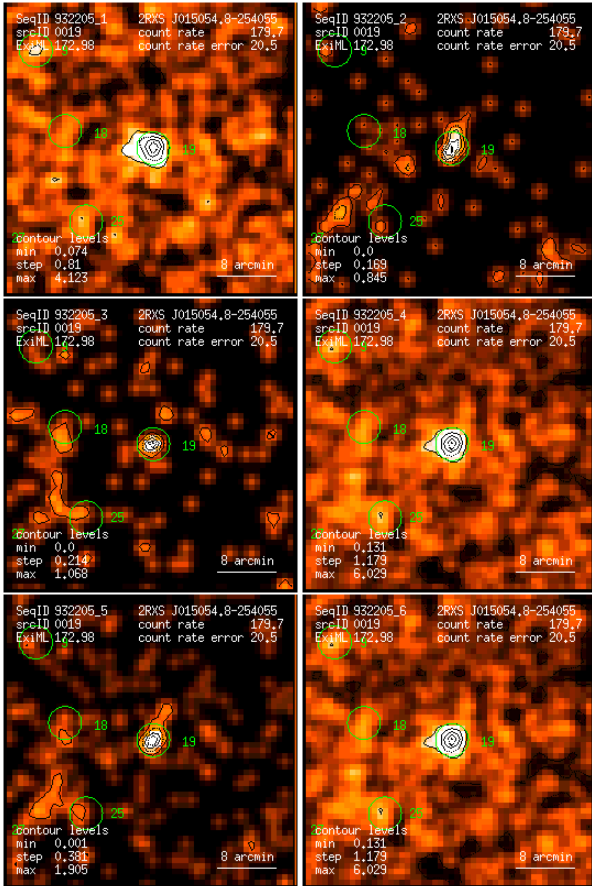
Figure 19: RASS 932205: detection 0019: band rate images, Gaussian filter: (1) PSPC channels 11 – 41, (2) 52 – 90, (3) 91 – 201, (4) 11 – 235, (5) 52 – 201, (6) 11 – 201. Broad band rates in counts/ks. Band rate contour levels in counts/ks/arcmin 2 .
