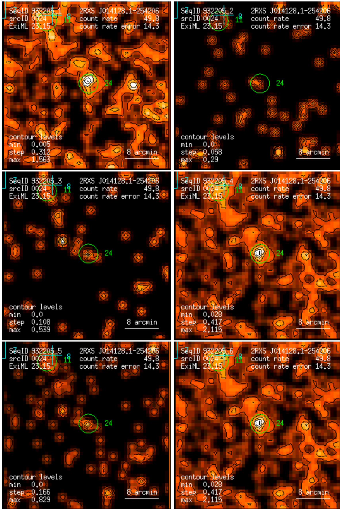
Figure 24: RASS 932205: detection 0024: band rate images, Gaussian filter: (1) PSPC channels 11 – 41, (2) 52 – 90, (3) 91 – 201, (4) 11 – 235, (5) 52 – 201, (6) 11 – 201. Broad band rates in counts/ks. Band rate contour levels in counts/ks/arcmin 2 .
