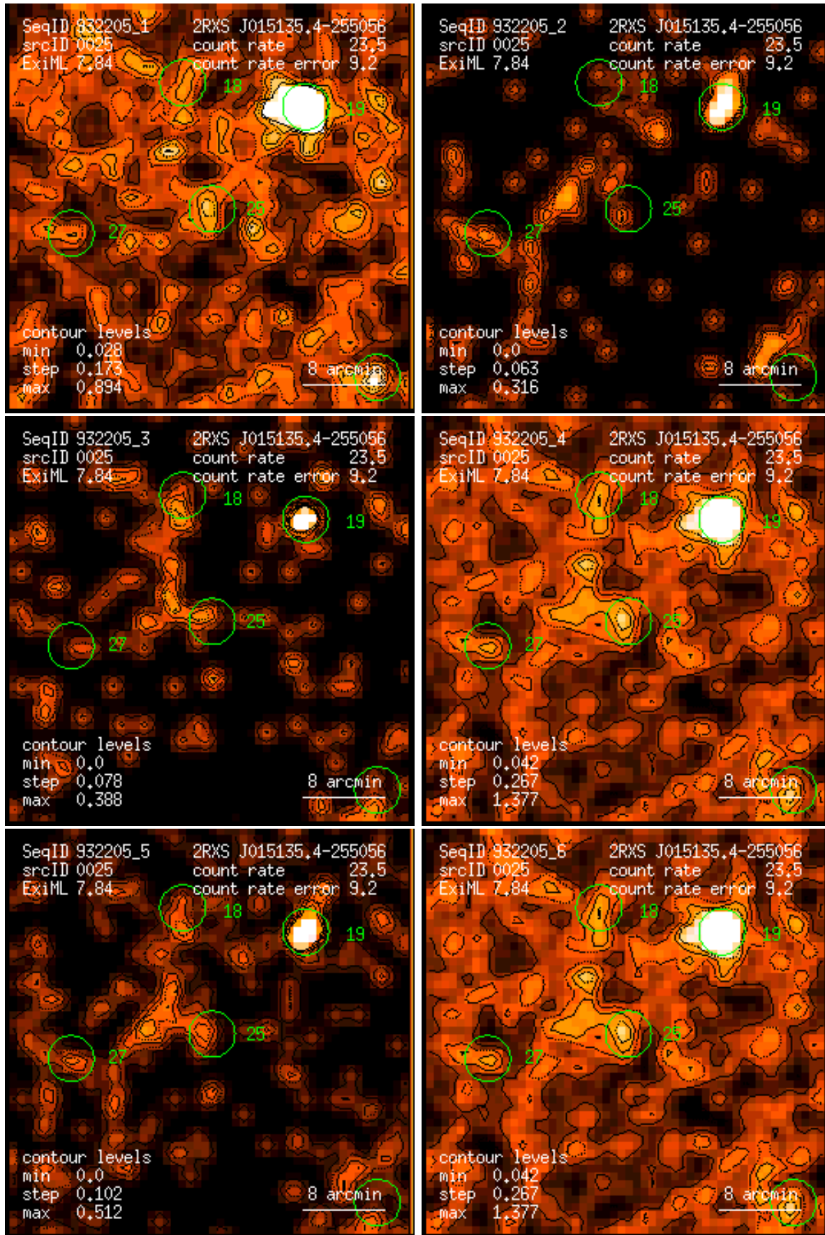
Figure 25: RASS 932205: detection 0025: band rate images, Gaussian filter: (1) PSPC channels 11 – 41, (2) 52 – 90, (3) 91 – 201, (4) 11 – 235, (5) 52 – 201, (6) 11 – 201. Broad band rates in counts/ks. Band rate contour levels in counts/ks/arcmin 2 .
