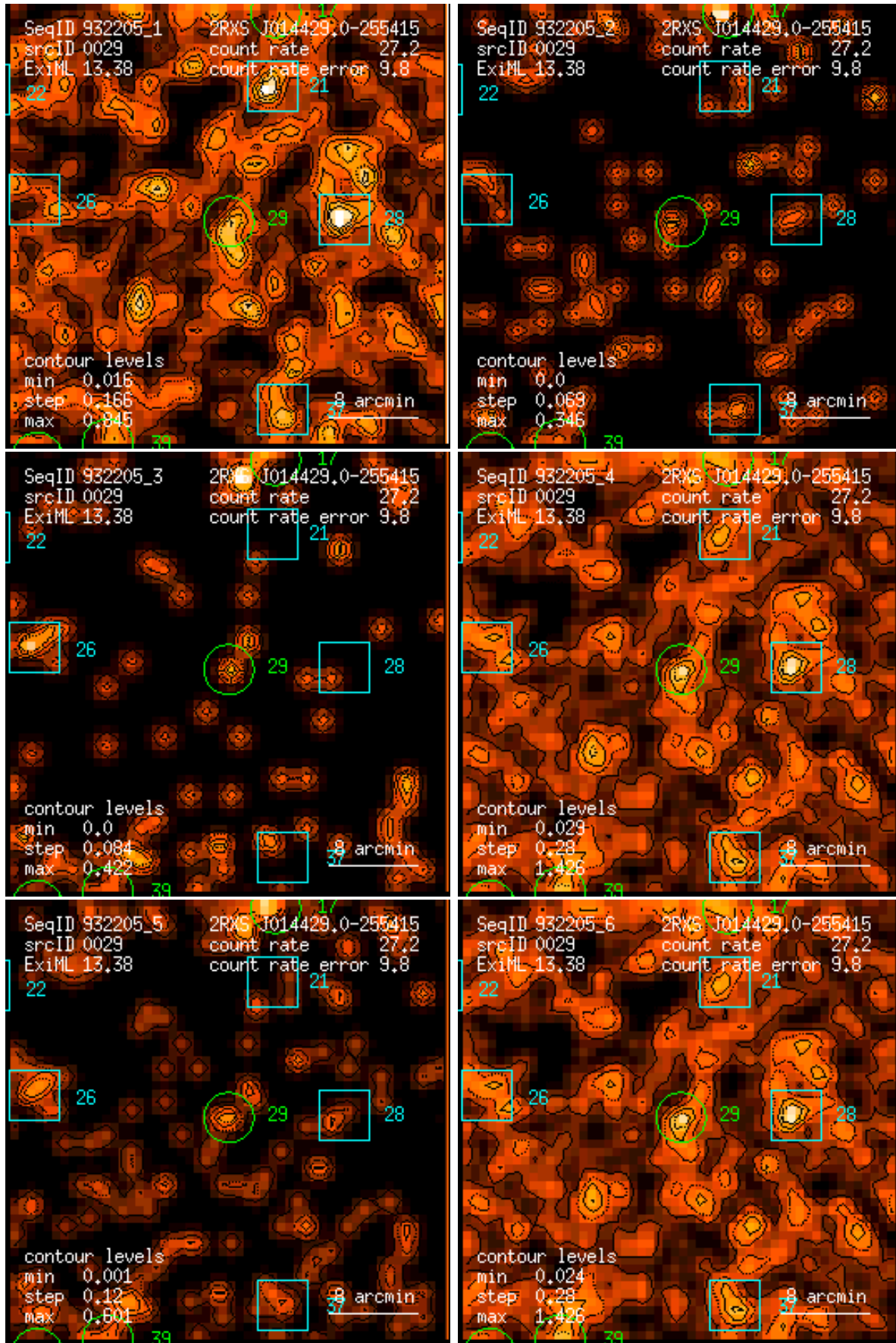
Figure 29: RASS 932205: detection 0029: band rate images, Gaussian filter: (1) PSPC channels 11 – 41, (2) 52 – 90, (3) 91 – 201, (4) 11 – 235, (5) 52 – 201, (6) 11 – 201. Broad band rates in counts/ks. Band rate contour levels in counts/ks/arcmin 2 .
