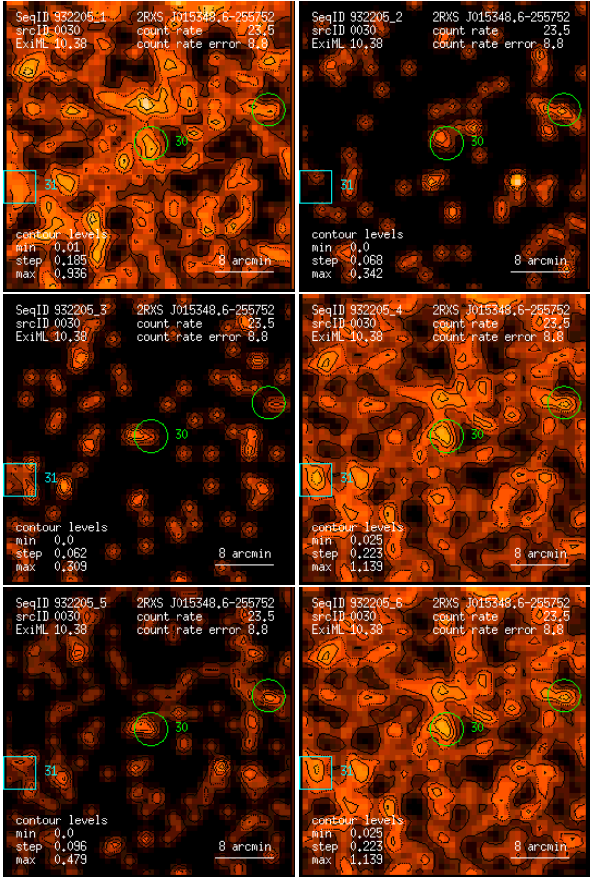
Figure 30: RASS 932205: detection 0030: band rate images, Gaussian filter: (1) PSPC channels 11 – 41, (2) 52 – 90, (3) 91 – 201, (4) 11 – 235, (5) 52 – 201, (6) 11 – 201. Broad band rates in counts/ks. Band rate contour levels in counts/ks/arcmin 2 .
