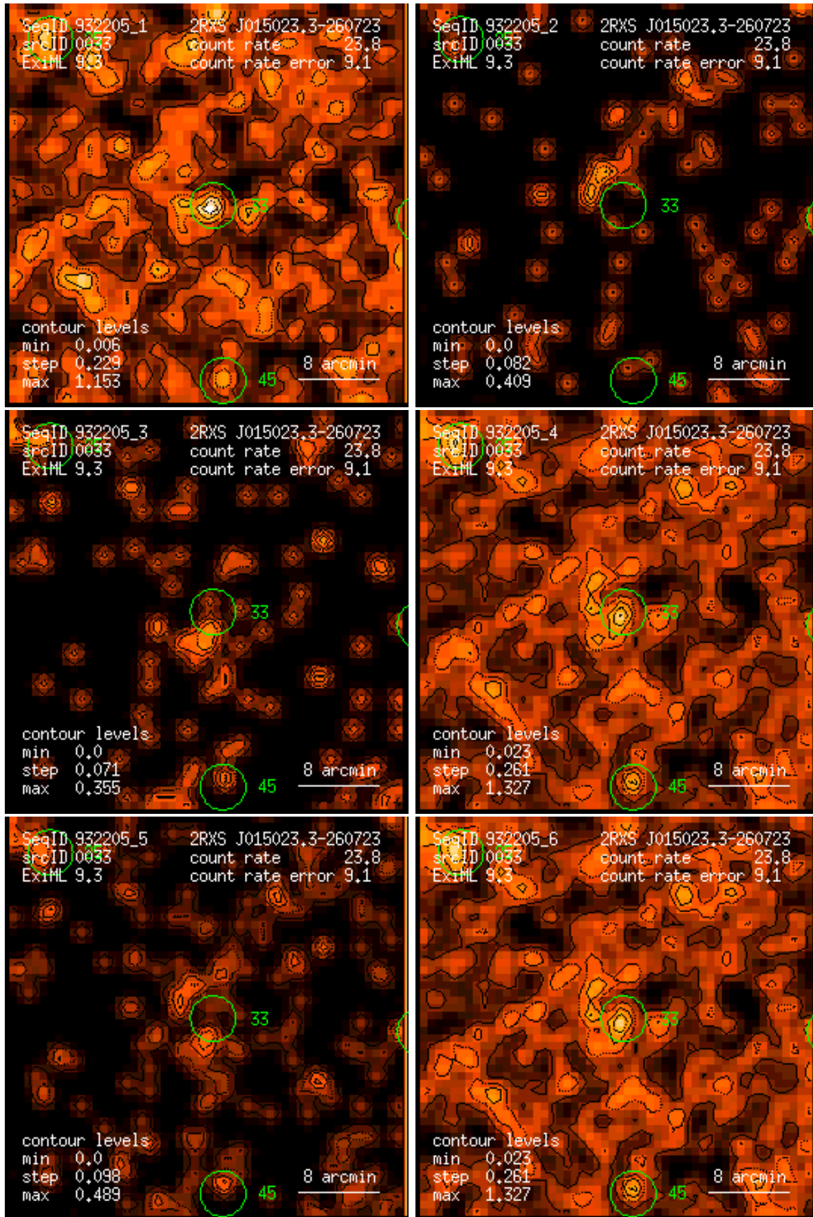
Figure 33: RASS 932205: detection 0033: band rate images, Gaussian filter: (1) PSPC channels 11 – 41, (2) 52 – 90, (3) 91 – 201, (4) 11 – 235, (5) 52 – 201, (6) 11 – 201. Broad band rates in counts/ks. Band rate contour levels in counts/ks/arcmin 2 .
