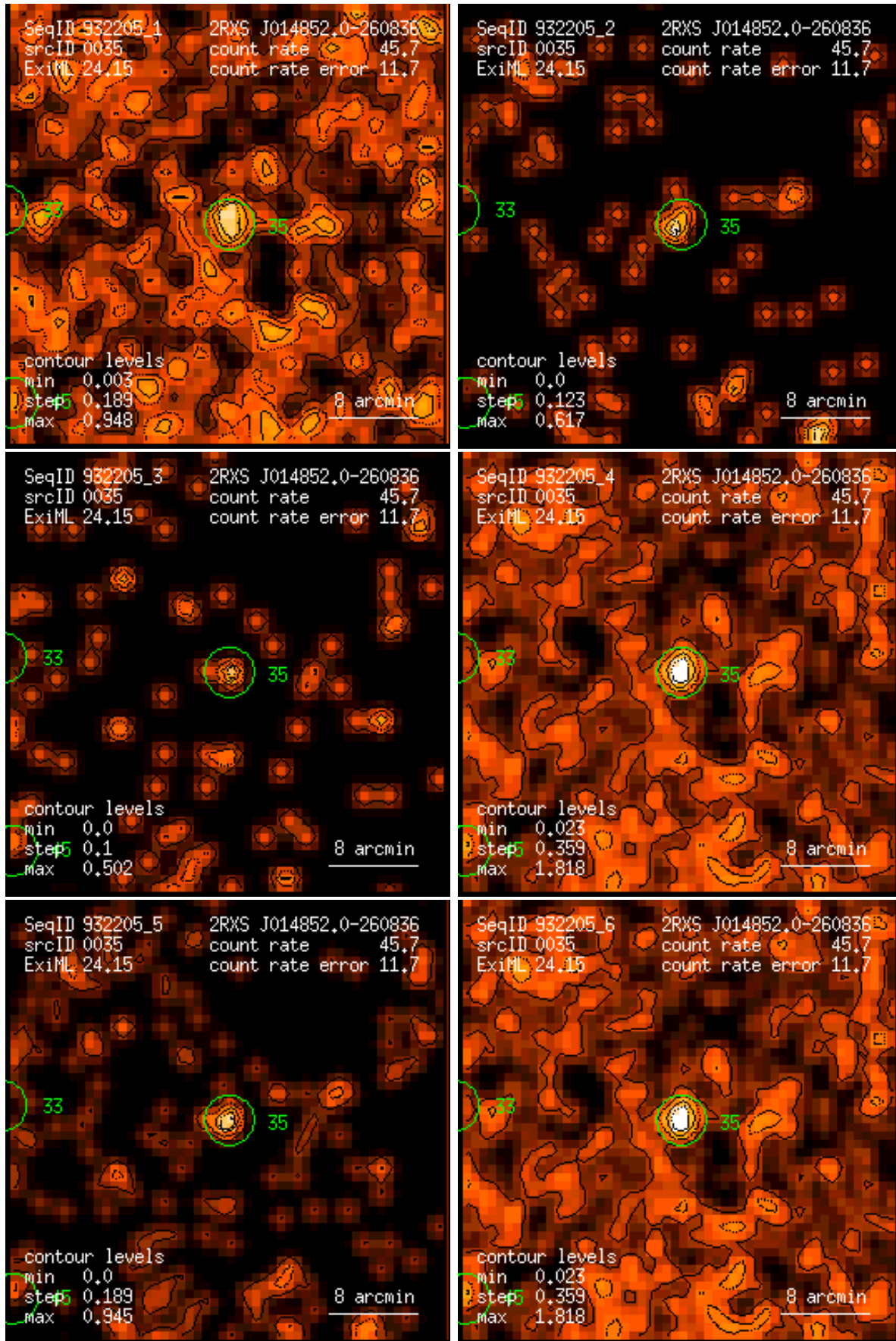
Figure 35: RASS 932205: detection 0035: band rate images, Gaussian filter: (1) PSPC channels 11 – 41, (2) 52 – 90, (3) 91 – 201, (4) 11 – 235, (5) 52 – 201, (6) 11 – 201. Broad band rates in counts/ks. Band rate contour levels in counts/ks/arcmin 2 .
