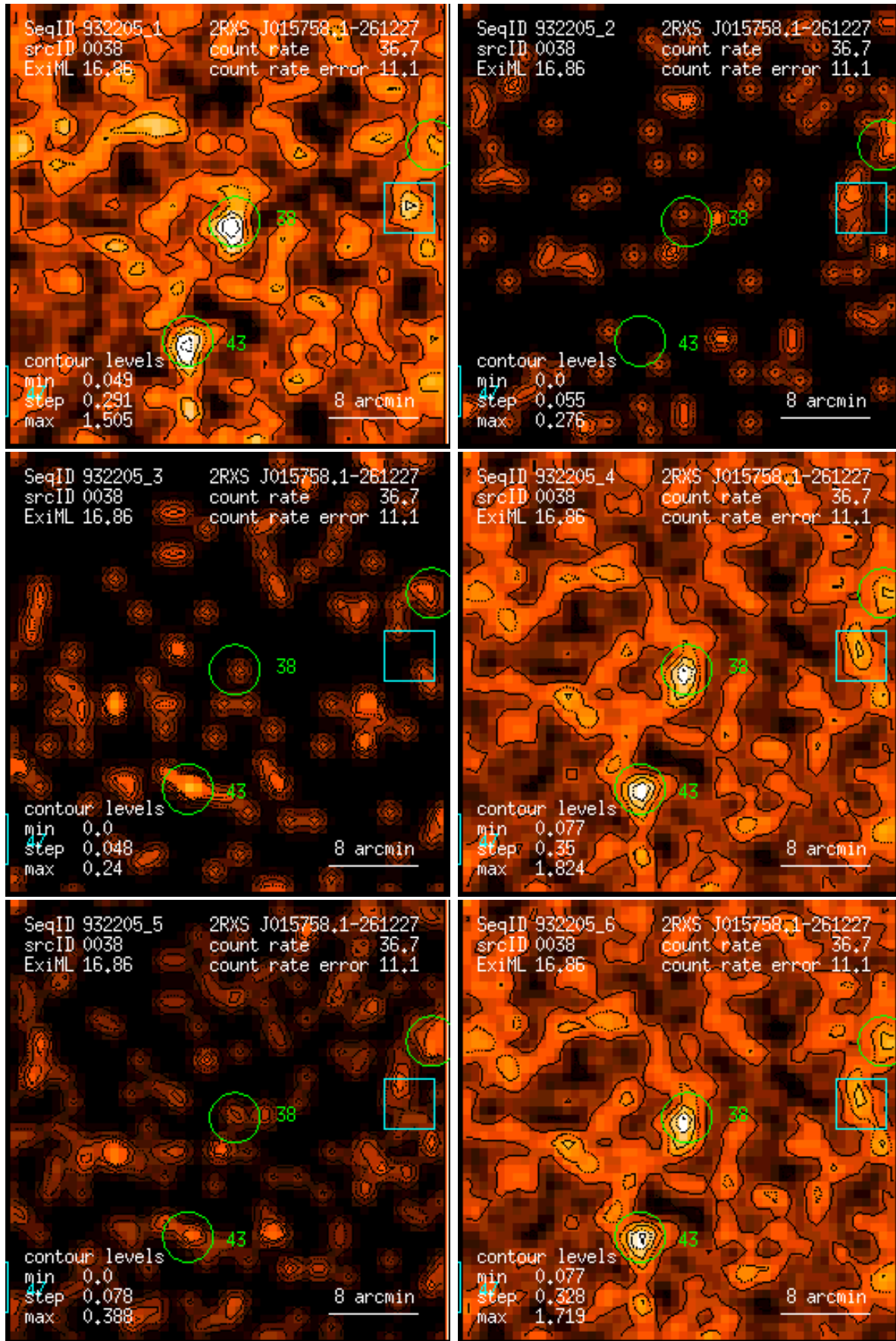
Figure 38: RASS 932205: detection 0038: band rate images, Gaussian filter: (1) PSPC channels 11 – 41, (2) 52 – 90, (3) 91 – 201, (4) 11 – 235, (5) 52 – 201, (6) 11 – 201. Broad band rates in counts/ks. Band rate contour levels in counts/ks/arcmin 2 .
