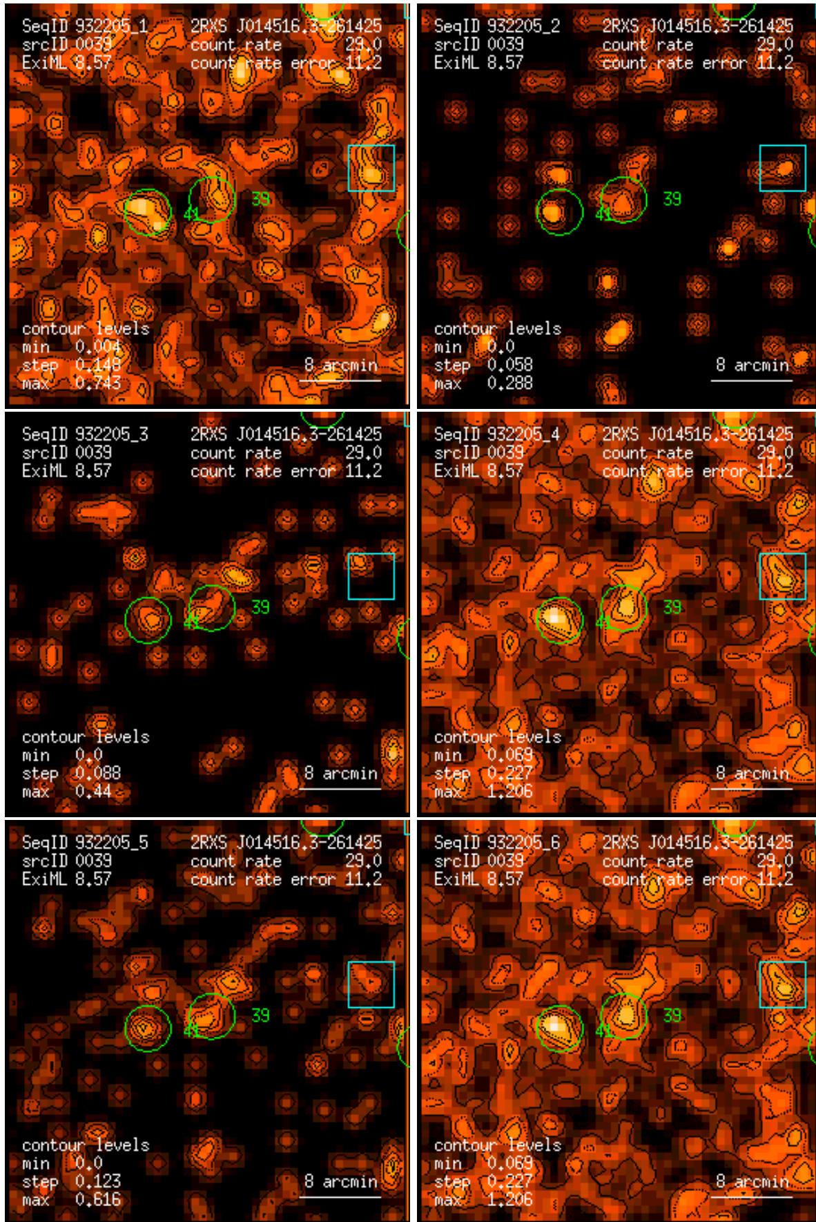
Figure 39: RASS 932205: detection 0039: band rate images, Gaussian filter: (1) PSPC channels 11 – 41, (2) 52 – 90, (3) 91 – 201, (4) 11 – 235, (5) 52 – 201, (6) 11 – 201. Broad band rates in counts/ks. Band rate contour levels in counts/ks/arcmin 2 .
