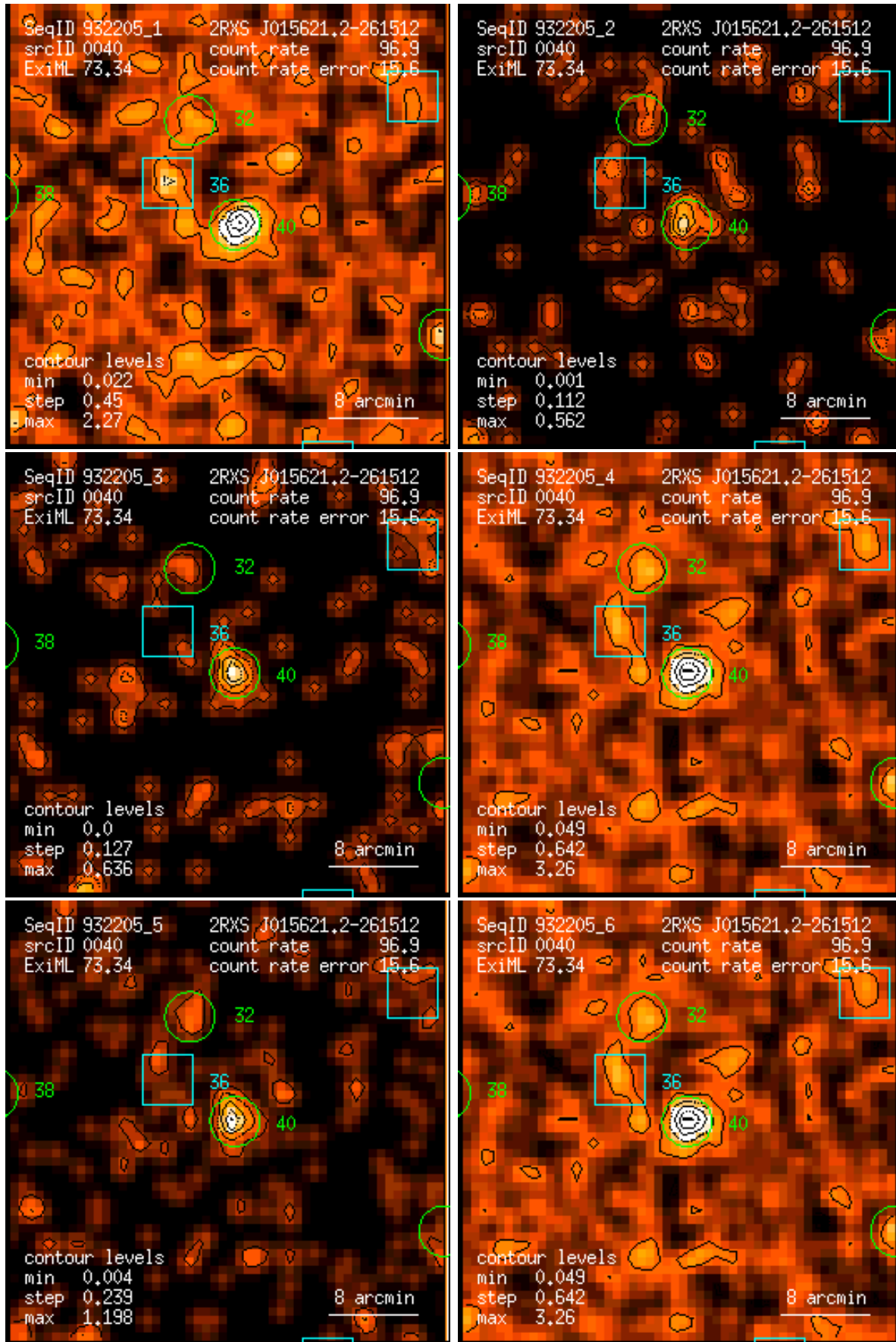
Figure 40: RASS 932205: detection 0040: band rate images, Gaussian filter: (1) PSPC channels 11 – 41, (2) 52 – 90, (3) 91 – 201, (4) 11 – 235, (5) 52 – 201, (6) 11 – 201. Broad band rates in counts/ks. Band rate contour levels in counts/ks/arcmin 2 .
