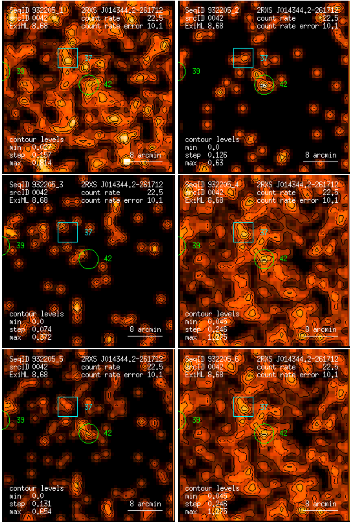
Figure 42: RASS 932205: detection 0042: band rate images, Gaussian filter: (1) PSPC channels 11 – 41, (2) 52 – 90, (3) 91 – 201, (4) 11 – 235, (5) 52 – 201, (6) 11 – 201. Broad band rates in counts/ks. Band rate contour levels in counts/ks/arcmin 2 .
