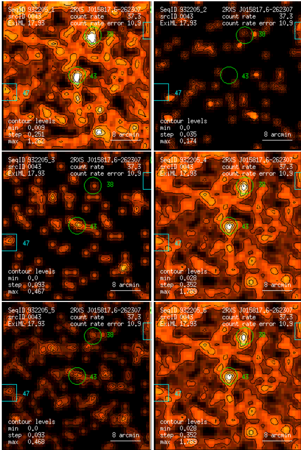
Figure 43: RASS 932205: detection 0043: band rate images, Gaussian filter: (1) PSPC channels 11 – 41, (2) 52 – 90, (3) 91 – 201, (4) 11 – 235, (5) 52 – 201, (6) 11 – 201. Broad band rates in counts/ks. Band rate contour levels in counts/ks/arcmin 2 .
