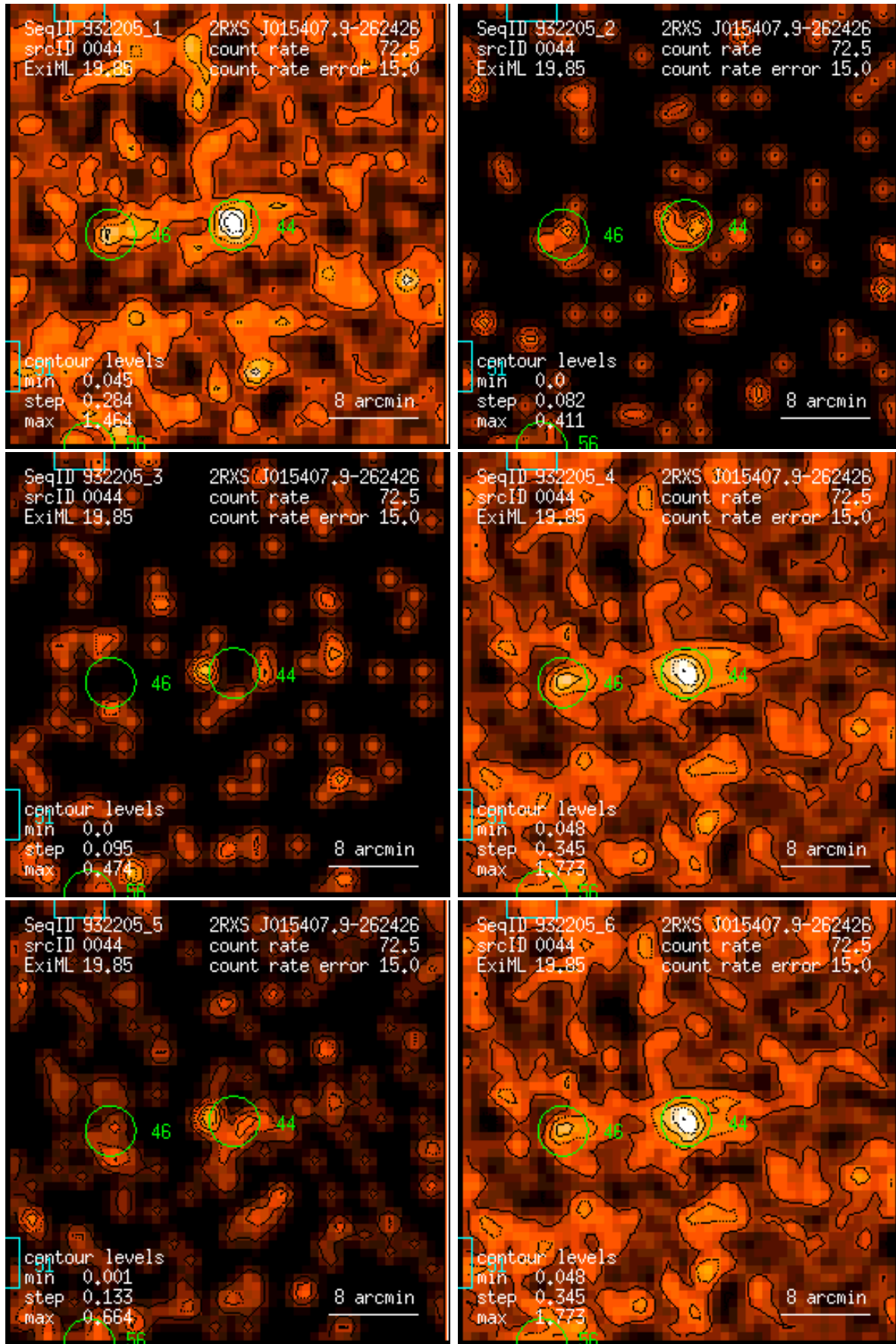
Figure 44: RASS 932205: detection 0044: band rate images, Gaussian filter: (1) PSPC channels 11 – 41, (2) 52 – 90, (3) 91 – 201, (4) 11 – 235, (5) 52 – 201, (6) 11 – 201. Broad band rates in counts/ks. Band rate contour levels in counts/ks/arcmin 2 .
