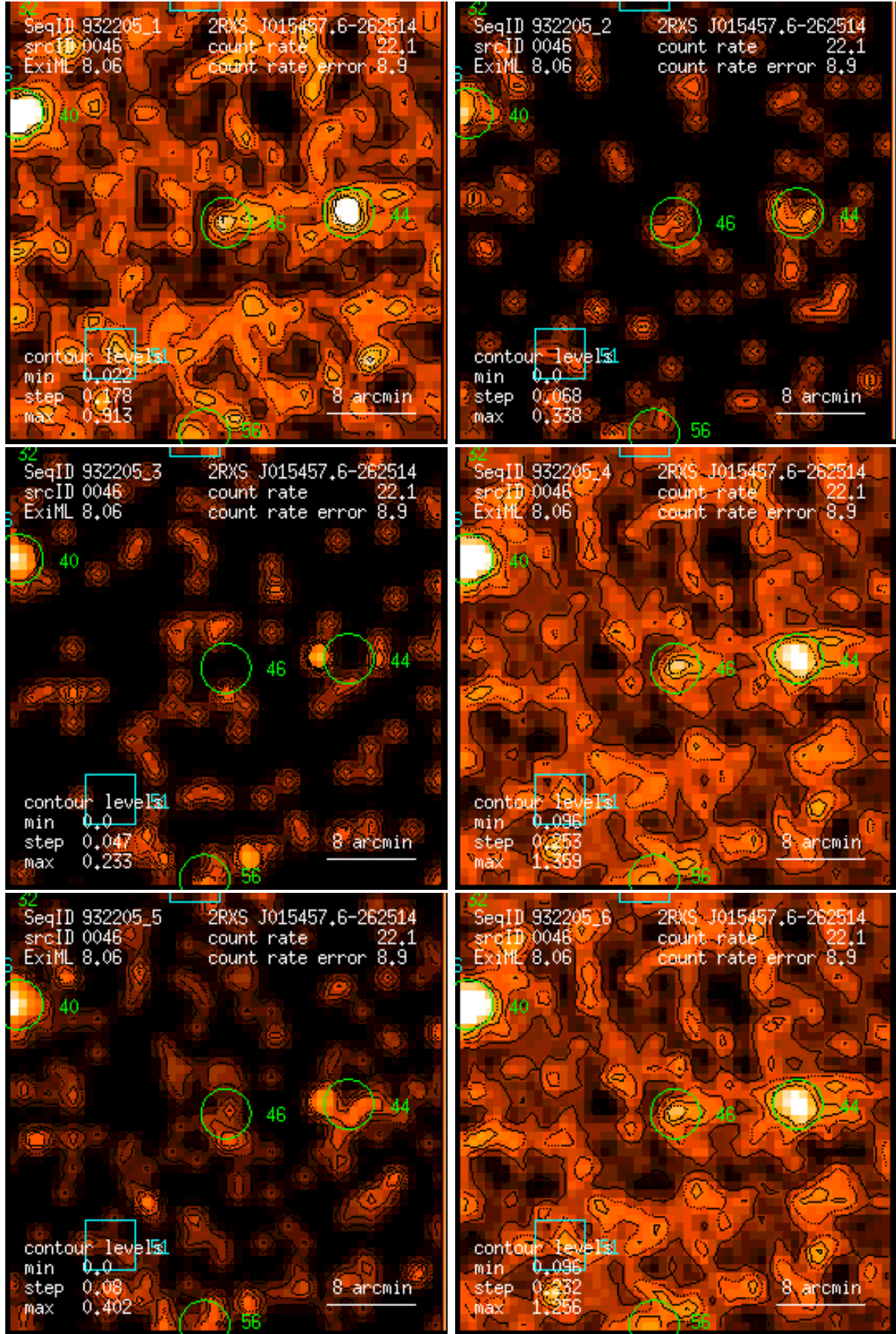
Figure 46: RASS 932205: detection 0046: band rate images, Gaussian filter: (1) PSPC channels 11 – 41, (2) 52 – 90, (3) 91 – 201, (4) 11 – 235, (5) 52 – 201, (6) 11 – 201. Broad band rates in counts/ks. Band rate contour levels in counts/ks/arcmin 2 .
