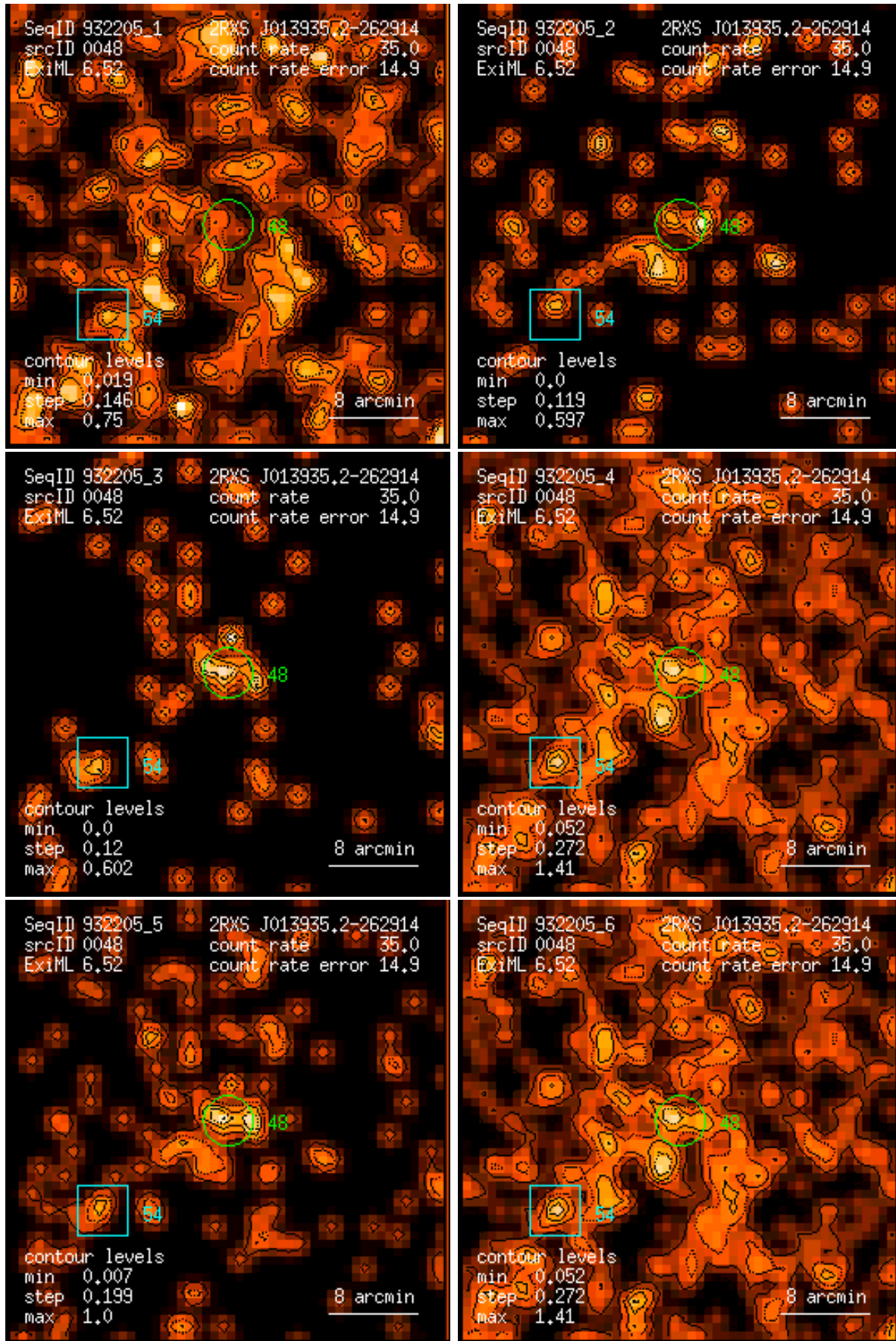
Figure 48: RASS 932205: detection 0048: band rate images, Gaussian filter: (1) PSPC channels 11 – 41, (2) 52 – 90, (3) 91 – 201, (4) 11 – 235, (5) 52 – 201, (6) 11 – 201. Broad band rates in counts/ks. Band rate contour levels in counts/ks/arcmin 2 .
