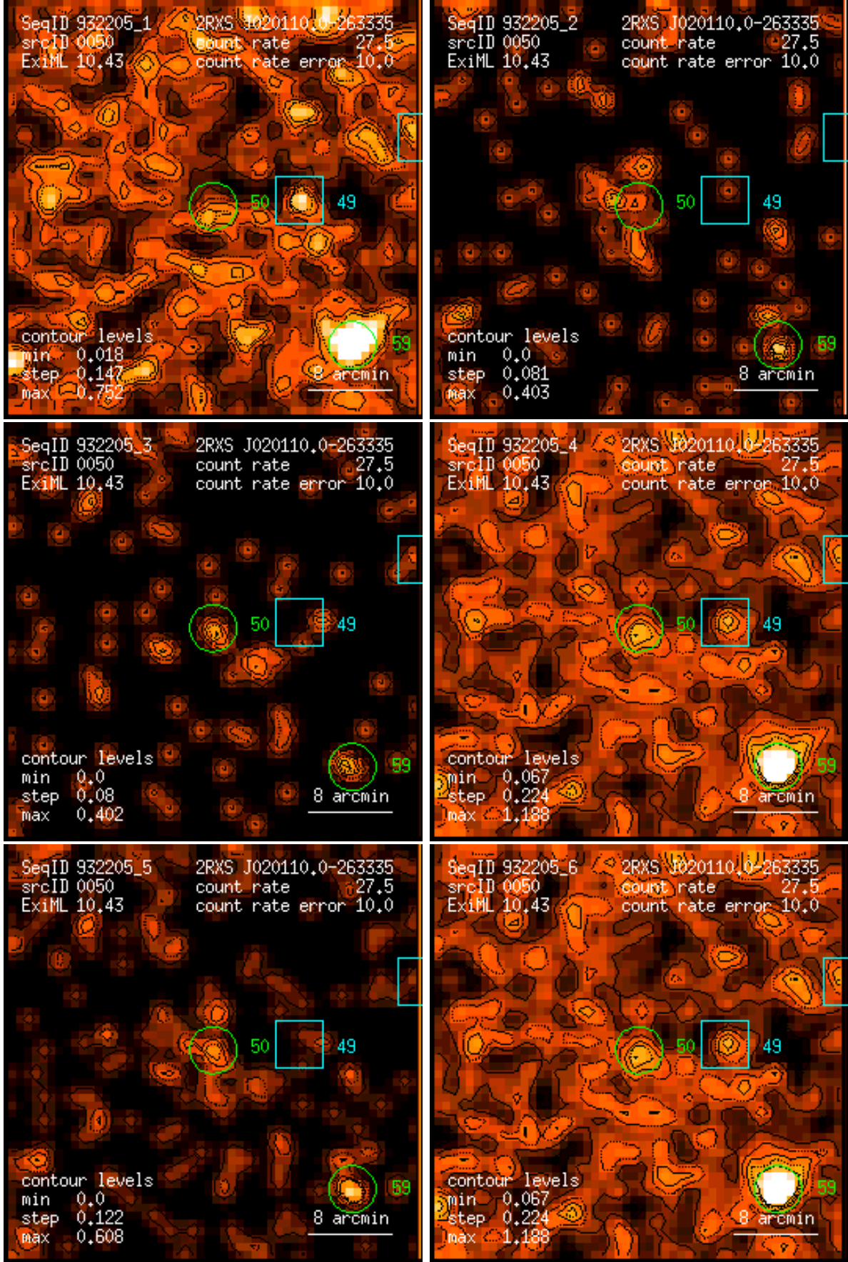
Figure 50: RASS 932205: detection 0050: band rate images, Gaussian filter: (1) PSPC channels 11 – 41, (2) 52 – 90, (3) 91 – 201, (4) 11 – 235, (5) 52 – 201, (6) 11 – 201. Broad band rates in counts/ks. Band rate contour levels in counts/ks/arcmin 2 .
