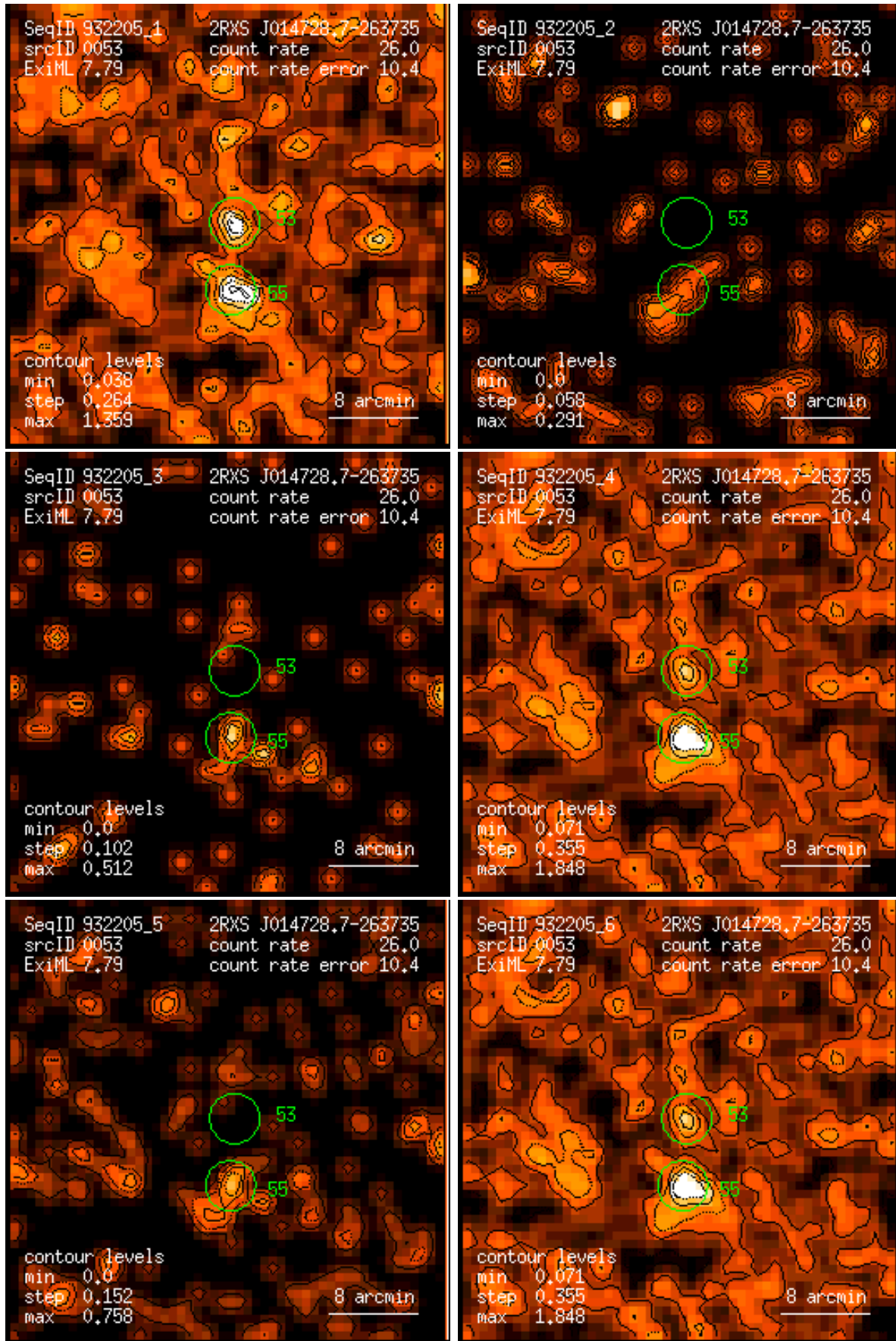
Figure 53: RASS 932205: detection 0053: band rate images, Gaussian filter: (1) PSPC channels 11 – 41, (2) 52 – 90, (3) 91 – 201, (4) 11 – 235, (5) 52 – 201, (6) 11 – 201. Broad band rates in counts/ks. Band rate contour levels in counts/ks/arcmin 2 .
