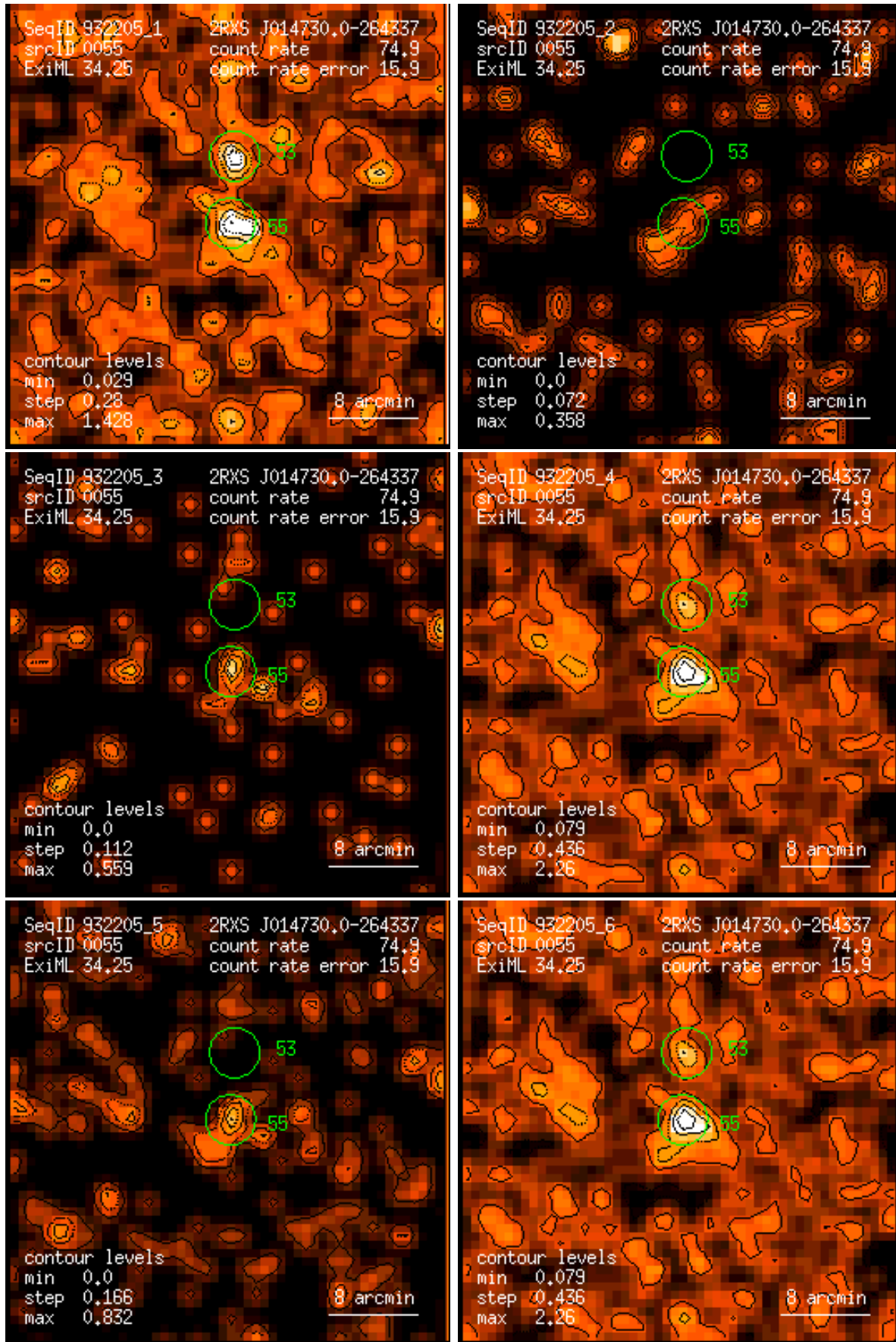
Figure 55: RASS 932205: detection 0055: band rate images, Gaussian filter: (1) PSPC channels 11 – 41, (2) 52 – 90, (3) 91 – 201, (4) 11 – 235, (5) 52 – 201, (6) 11 – 201. Broad band rates in counts/ks. Band rate contour levels in counts/ks/arcmin 2 .
