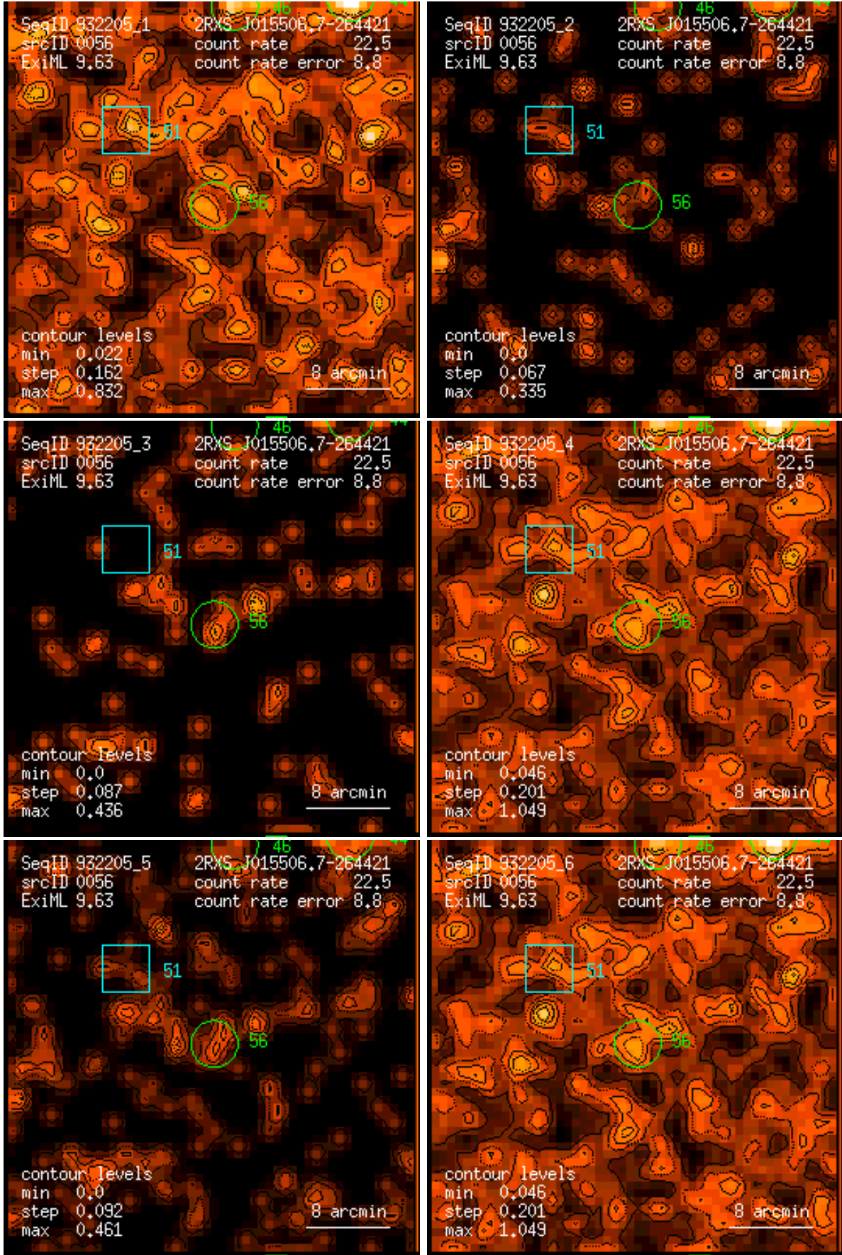
Figure 56: RASS 932205: detection 0056: band rate images, Gaussian filter: (1) PSPC channels 11 – 41, (2) 52 – 90, (3) 91 – 201, (4) 11 – 235, (5) 52 – 201, (6) 11 – 201. Broad band rates in counts/ks. Band rate contour levels in counts/ks/arcmin 2 .
