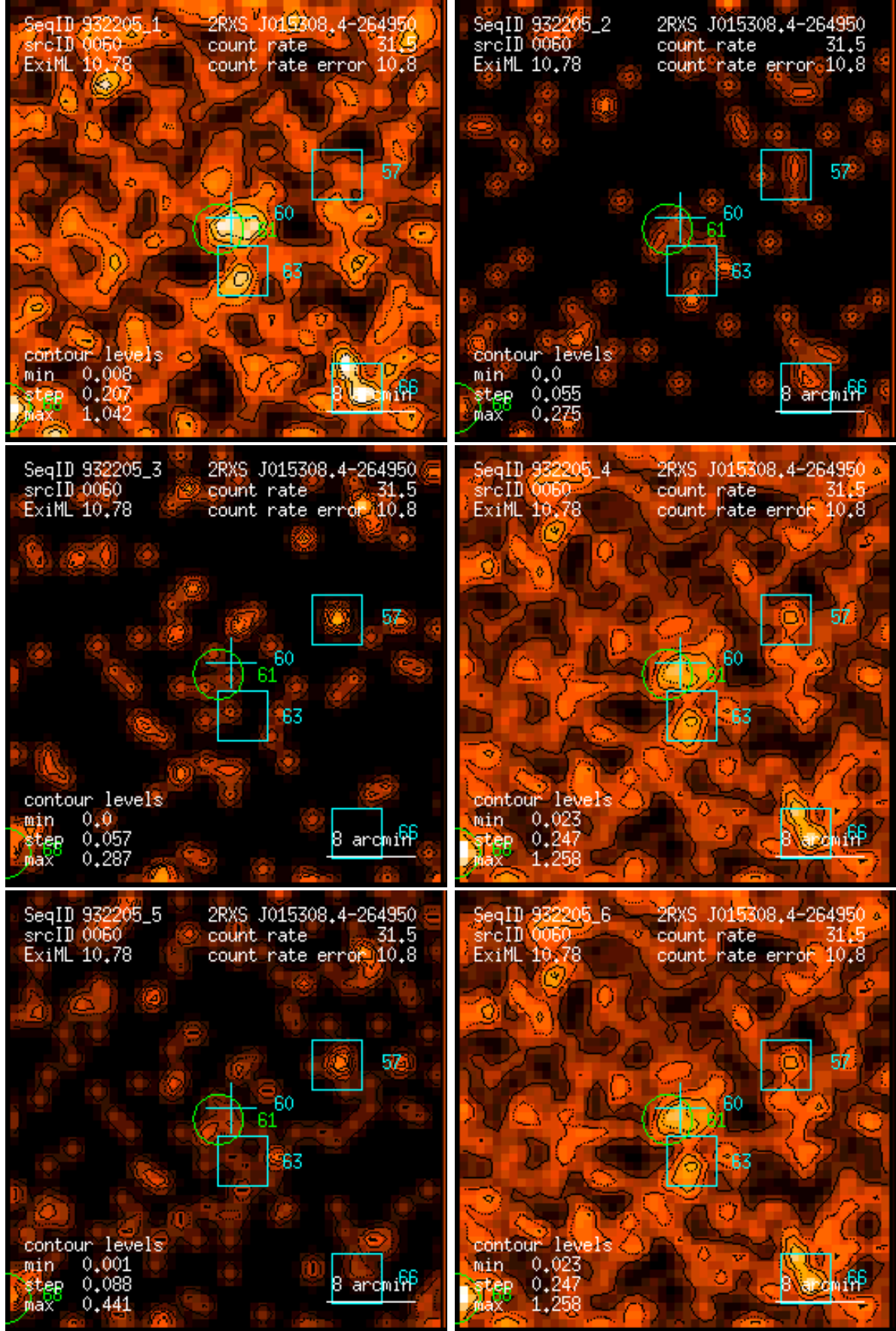
Figure 60: RASS 932205: detection 0060: band rate images, Gaussian filter: (1) PSPC channels 11 – 41, (2) 52 – 90, (3) 91 – 201, (4) 11 – 235, (5) 52 – 201, (6) 11 – 201. Broad band rates in counts/ks. Band rate contour levels in counts/ks/arcmin 2 .
