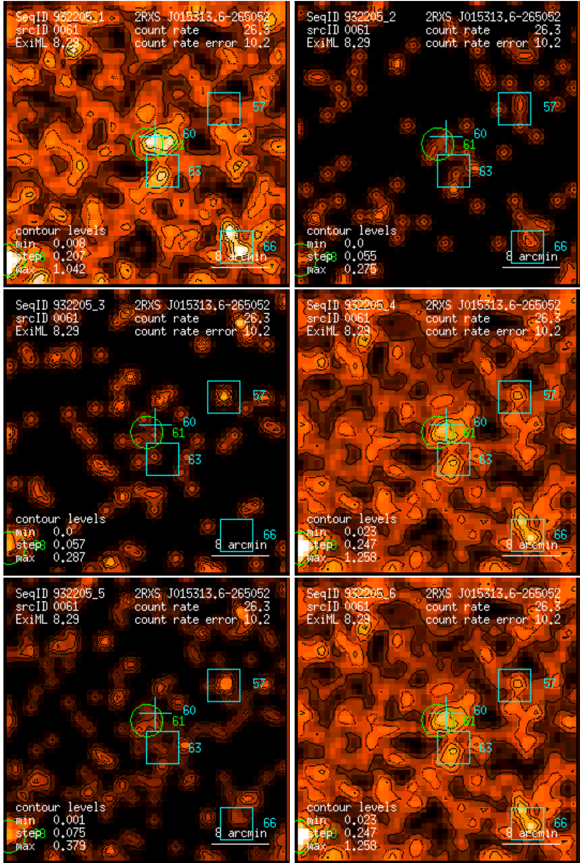
Figure 61: RASS 932205: detection 0061: band rate images, Gaussian filter: (1) PSPC channels 11 – 41, (2) 52 – 90, (3) 91 – 201, (4) 11 – 235, (5) 52 – 201, (6) 11 – 201. Broad band rates in counts/ks. Band rate contour levels in counts/ks/arcmin 2 .
