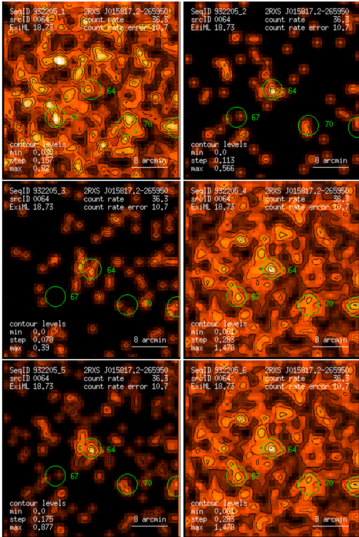
Figure 64: RASS 932205: detection 0064: band rate images, Gaussian filter: (1) PSPC channels 11 – 41, (2) 52 – 90, (3) 91 – 201, (4) 11 – 235, (5) 52 – 201, (6) 11 – 201. Broad band rates in counts/ks. Band rate contour levels in counts/ks/arcmin 2 .
