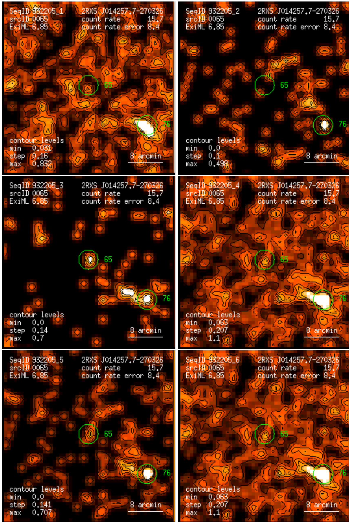
Figure 65: RASS 932205: detection 0065: band rate images, Gaussian filter: (1) PSPC channels 11 – 41, (2) 52 – 90, (3) 91 – 201, (4) 11 – 235, (5) 52 – 201, (6) 11 – 201. Broad band rates in counts/ks. Band rate contour levels in counts/ks/arcmin 2 .
