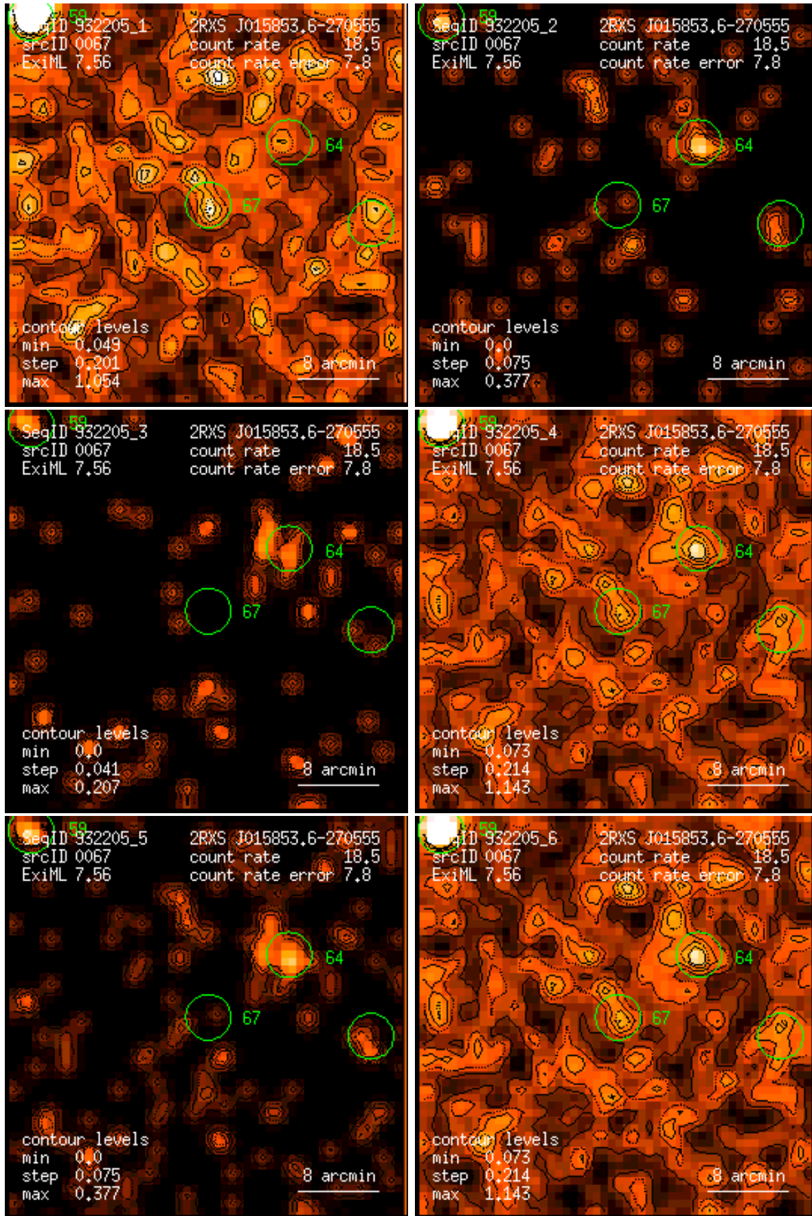
Figure 67: RASS 932205: detection 0067: band rate images, Gaussian filter: (1) PSPC channels 11 – 41, (2) 52 – 90, (3) 91 – 201, (4) 11 – 235, (5) 52 – 201, (6) 11 – 201. Broad band rates in counts/ks. Band rate contour levels in counts/ks/arcmin 2 .
