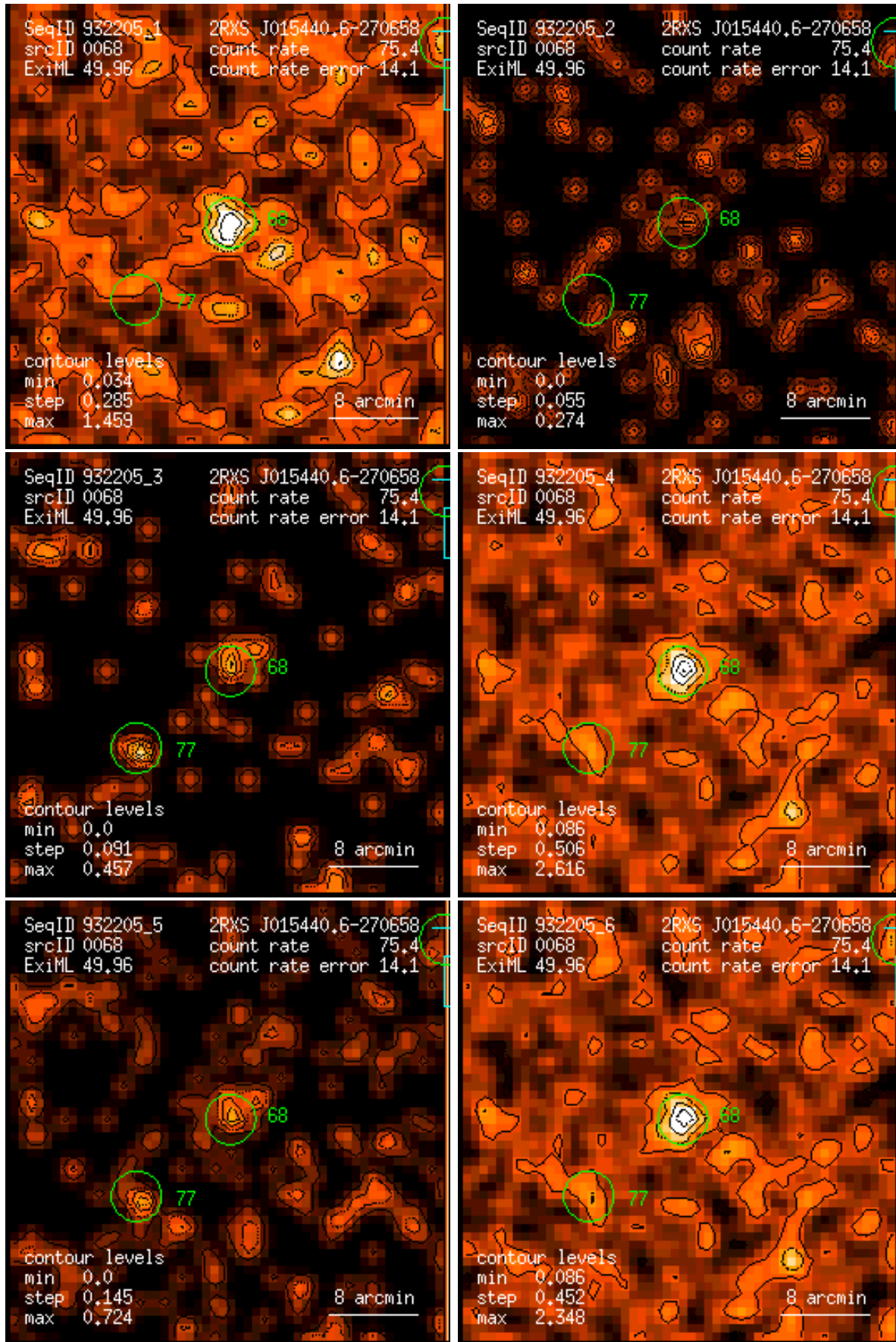
Figure 68: RASS 932205: detection 0068: band rate images, Gaussian filter: (1) PSPC channels 11 – 41, (2) 52 – 90, (3) 91 – 201, (4) 11 – 235, (5) 52 – 201, (6) 11 – 201. Broad band rates in counts/ks. Band rate contour levels in counts/ks/arcmin 2 .
