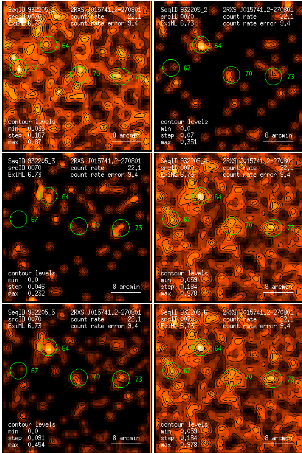
Figure 70: RASS 932205: detection 0070: band rate images, Gaussian filter: (1) PSPC channels 11 – 41, (2) 52 – 90, (3) 91 – 201, (4) 11 – 235, (5) 52 – 201, (6) 11 – 201. Broad band rates in counts/ks. Band rate contour levels in counts/ks/arcmin 2 .
