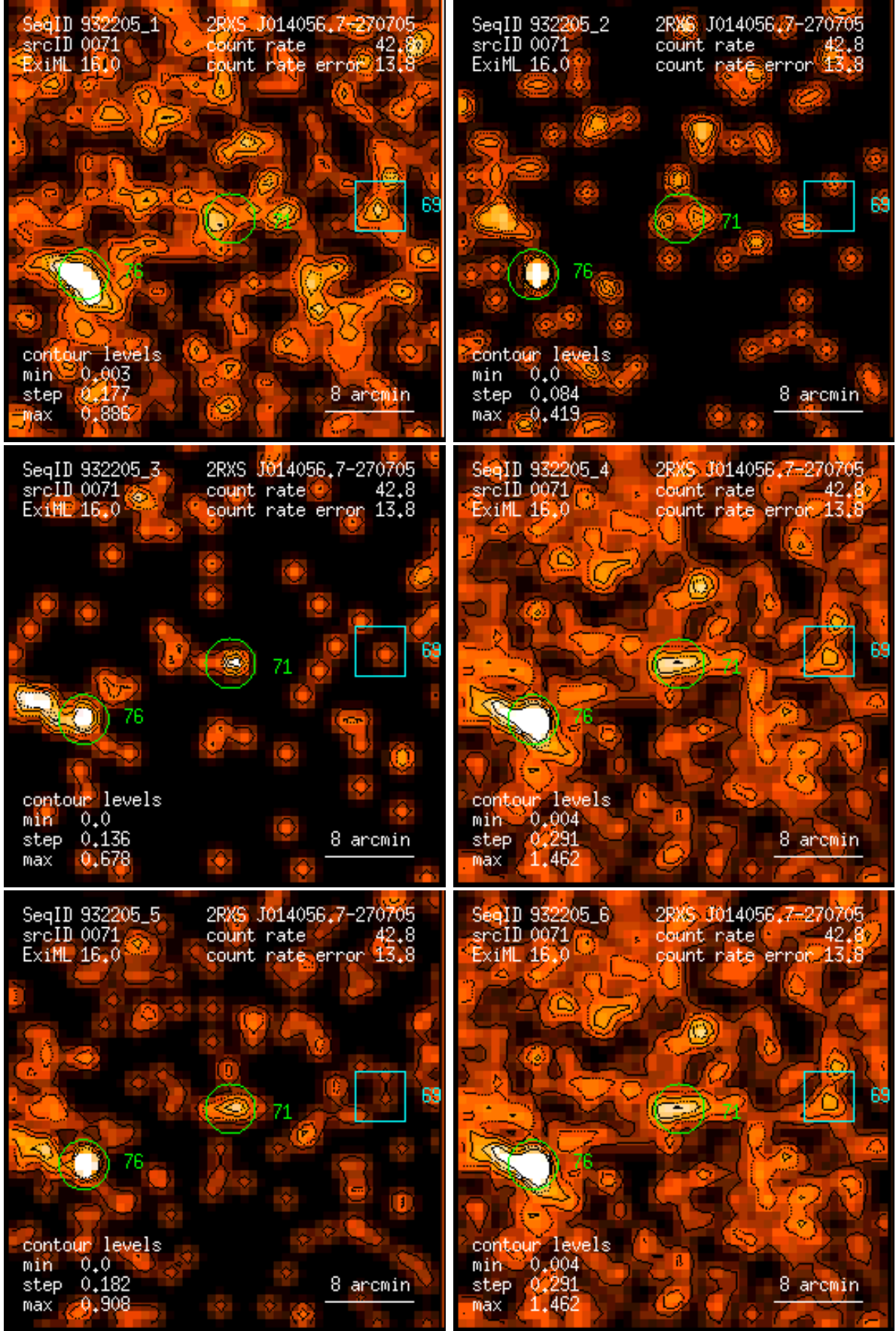
Figure 71: RASS 932205: detection 0071: band rate images, Gaussian filter: (1) PSPC channels 11 – 41, (2) 52 – 90, (3) 91 – 201, (4) 11 – 235, (5) 52 – 201, (6) 11 – 201. Broad band rates in counts/ks. Band rate contour levels in counts/ks/arcmin 2 .
