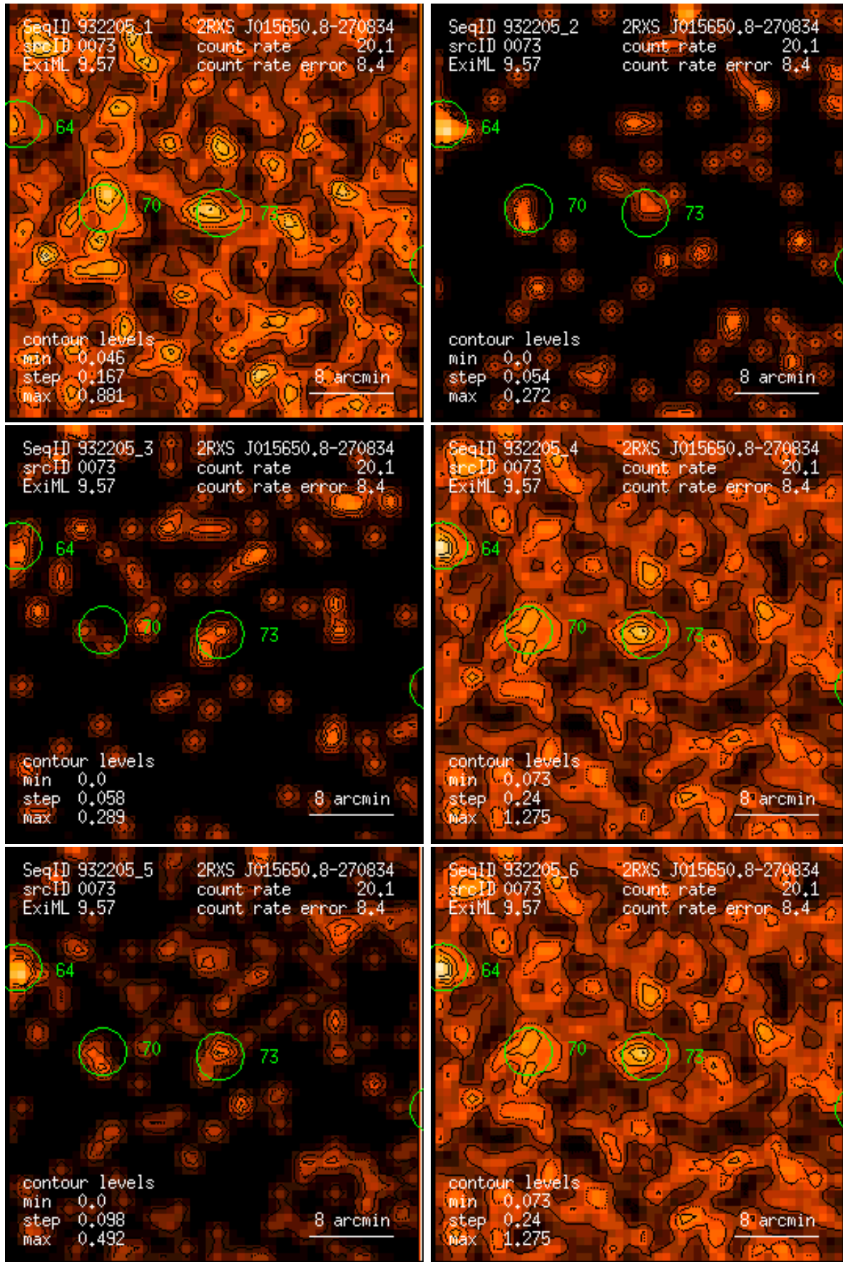
Figure 73: RASS 932205: detection 0073: band rate images, Gaussian filter: (1) PSPC channels 11 – 41, (2) 52 – 90, (3) 91 – 201, (4) 11 – 235, (5) 52 – 201, (6) 11 – 201. Broad band rates in counts/ks. Band rate contour levels in counts/ks/arcmin 2 .
