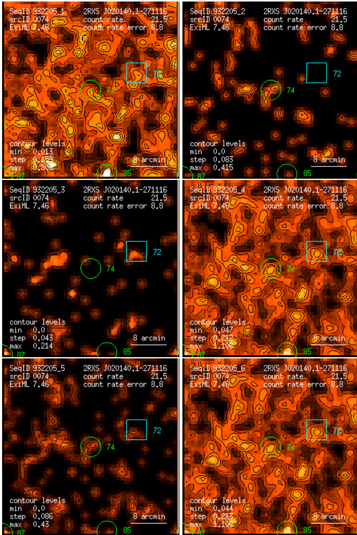
Figure 74: RASS 932205: detection 0074: band rate images, Gaussian filter: (1) PSPC channels 11 – 41, (2) 52 – 90, (3) 91 – 201, (4) 11 – 235, (5) 52 – 201, (6) 11 – 201. Broad band rates in counts/ks. Band rate contour levels in counts/ks/arcmin 2 .
