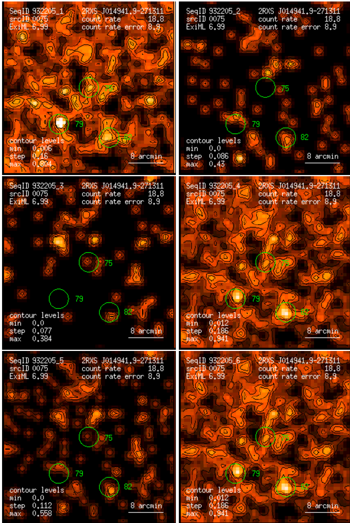
Figure 75: RASS 932205: detection 0075: band rate images, Gaussian filter: (1) PSPC channels 11 – 41, (2) 52 – 90, (3) 91 – 201, (4) 11 – 235, (5) 52 – 201, (6) 11 – 201. Broad band rates in counts/ks. Band rate contour levels in counts/ks/arcmin 2 .
