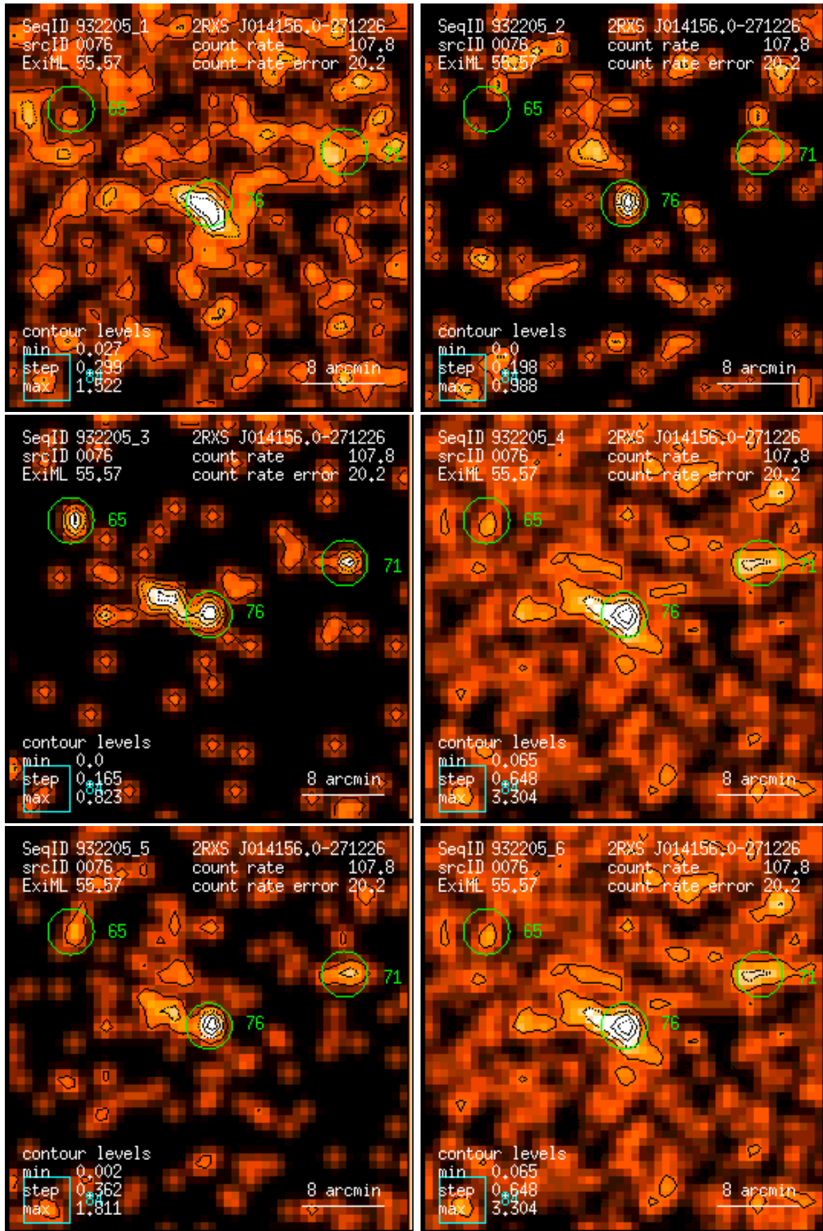
Figure 76: RASS 932205: detection 0076: band rate images, Gaussian filter: (1) PSPC channels 11 – 41, (2) 52 – 90, (3) 91 – 201, (4) 11 – 235, (5) 52 – 201, (6) 11 – 201. Broad band rates in counts/ks. Band rate contour levels in counts/ks/arcmin 2 .
