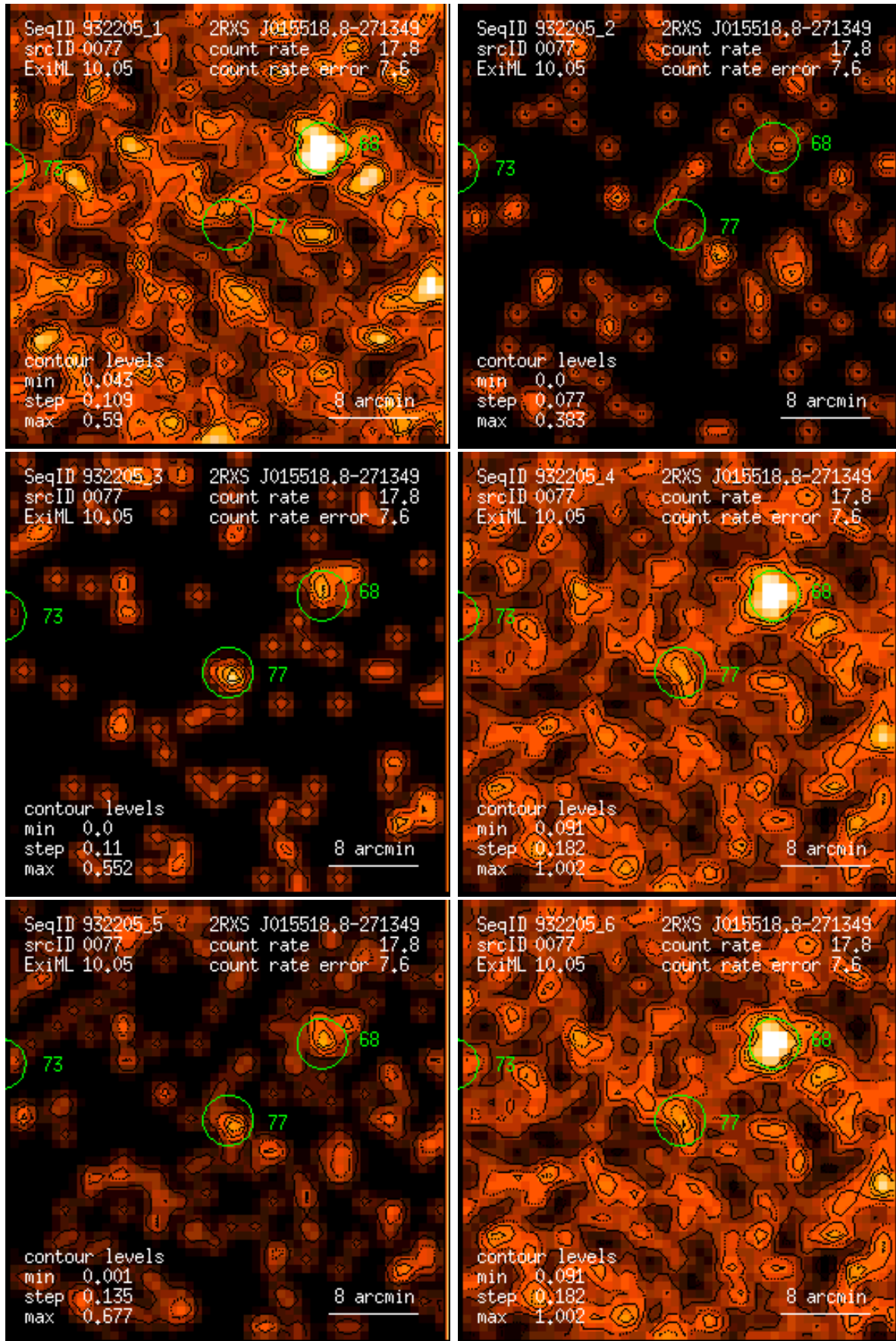
Figure 77: RASS 932205: detection 0077: band rate images, Gaussian filter: (1) PSPC channels 11 – 41, (2) 52 – 90, (3) 91 – 201, (4) 11 – 235, (5) 52 – 201, (6) 11 – 201. Broad band rates in counts/ks. Band rate contour levels in counts/ks/arcmin 2 .
