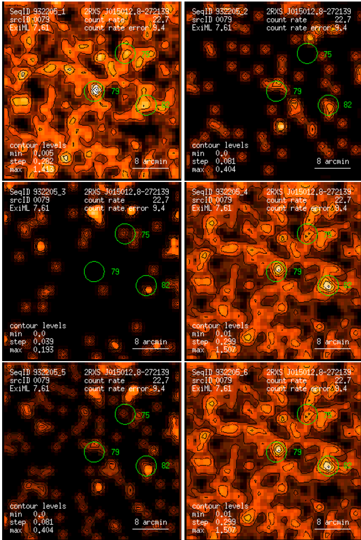
Figure 79: RASS 932205: detection 0079: band rate images, Gaussian filter: (1) PSPC channels 11 – 41, (2) 52 – 90, (3) 91 – 201, (4) 11 – 235, (5) 52 – 201, (6) 11 – 201. Broad band rates in counts/ks. Band rate contour levels in counts/ks/arcmin 2 .
