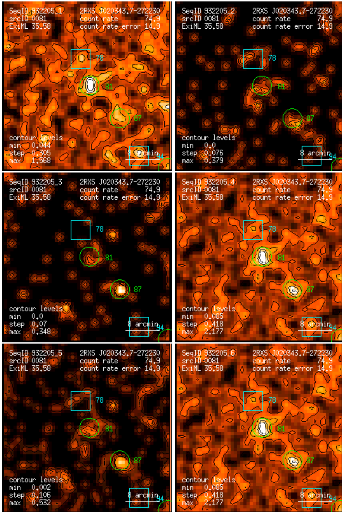
Figure 81: RASS 932205: detection 0081: band rate images, Gaussian filter: (1) PSPC channels 11 – 41, (2) 52 – 90, (3) 91 – 201, (4) 11 – 235, (5) 52 – 201, (6) 11 – 201. Broad band rates in counts/ks. Band rate contour levels in counts/ks/arcmin 2 .
