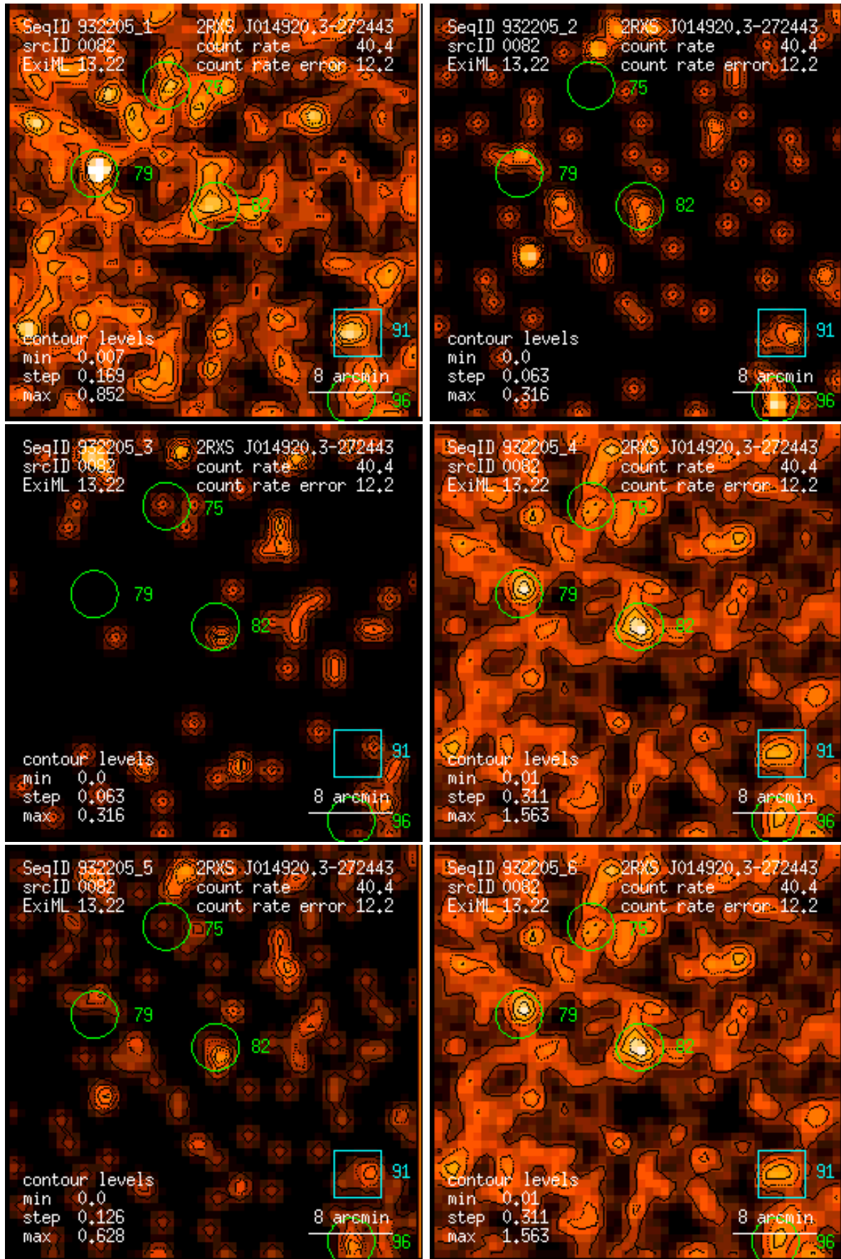
Figure 82: RASS 932205: detection 0082: band rate images, Gaussian filter: (1) PSPC channels 11 – 41, (2) 52 – 90, (3) 91 – 201, (4) 11 – 235, (5) 52 – 201, (6) 11 – 201. Broad band rates in counts/ks. Band rate contour levels in counts/ks/arcmin 2 .
