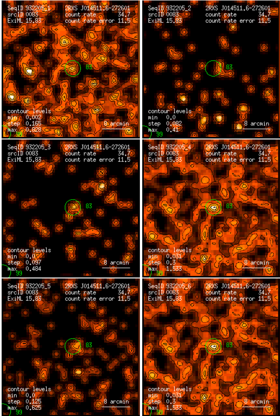
Figure 83: RASS 932205: detection 0083: band rate images, Gaussian filter: (1) PSPC channels 11 – 41, (2) 52 – 90, (3) 91 – 201, (4) 11 – 235, (5) 52 – 201, (6) 11 – 201. Broad band rates in counts/ks. Band rate contour levels in counts/ks/arcmin 2 .
