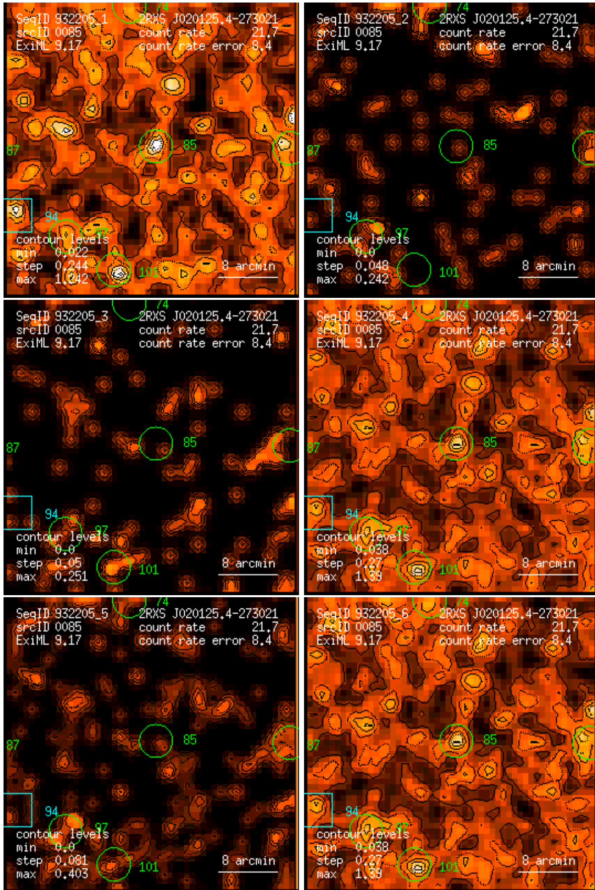
Figure 85: RASS 932205: detection 0085: band rate images, Gaussian filter: (1) PSPC channels 11 – 41, (2) 52 – 90, (3) 91 – 201, (4) 11 – 235, (5) 52 – 201, (6) 11 – 201. Broad band rates in counts/ks. Band rate contour levels in counts/ks/arcmin 2 .
