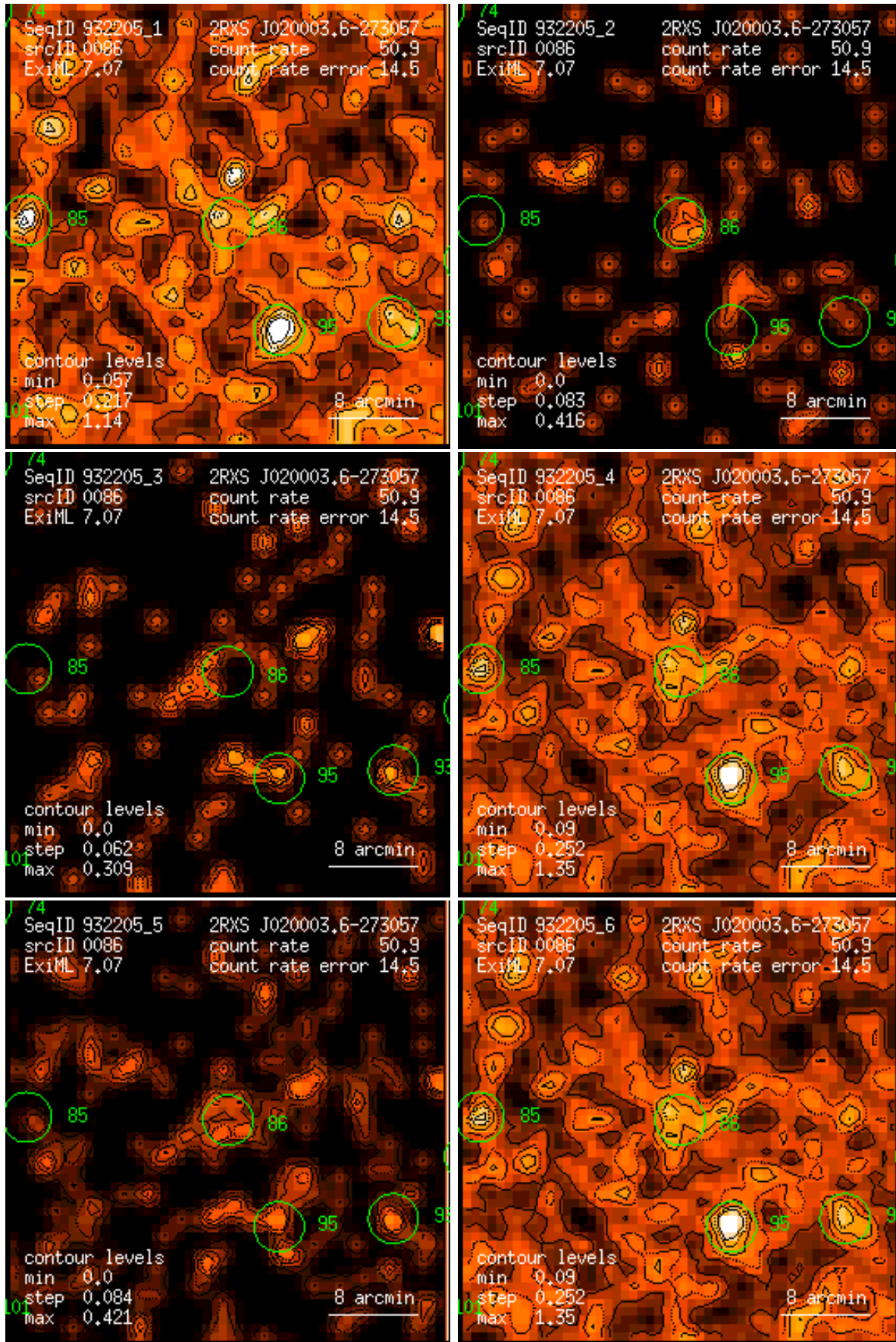
Figure 86: RASS 932205: detection 0086: band rate images, Gaussian filter: (1) PSPC channels 11 – 41, (2) 52 – 90, (3) 91 – 201, (4) 11 – 235, (5) 52 – 201, (6) 11 – 201. Broad band rates in counts/ks. Band rate contour levels in counts/ks/arcmin 2 .
