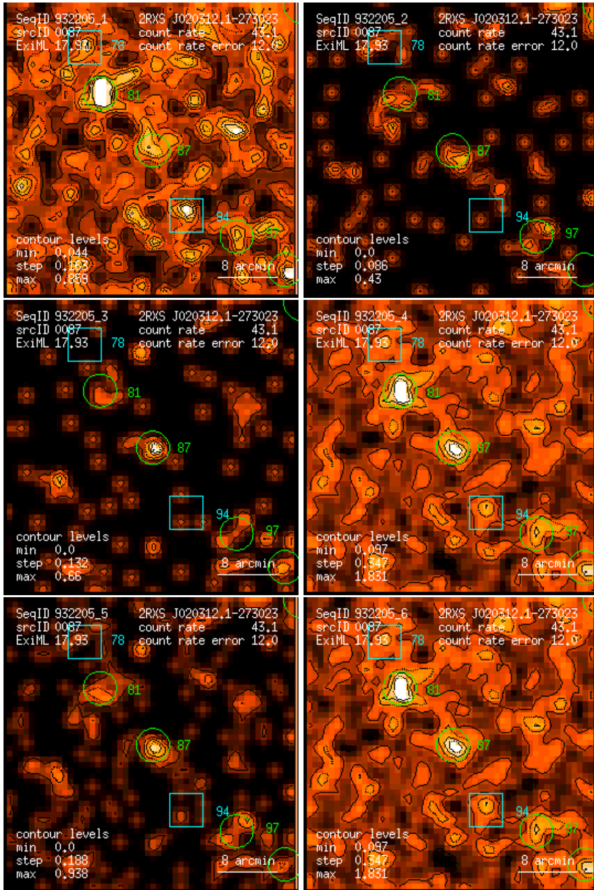
Figure 87: RASS 932205: detection 0087: band rate images, Gaussian filter: (1) PSPC channels 11 – 41, (2) 52 – 90, (3) 91 – 201, (4) 11 – 235, (5) 52 – 201, (6) 11 – 201. Broad band rates in counts/ks. Band rate contour levels in counts/ks/arcmin 2 .
