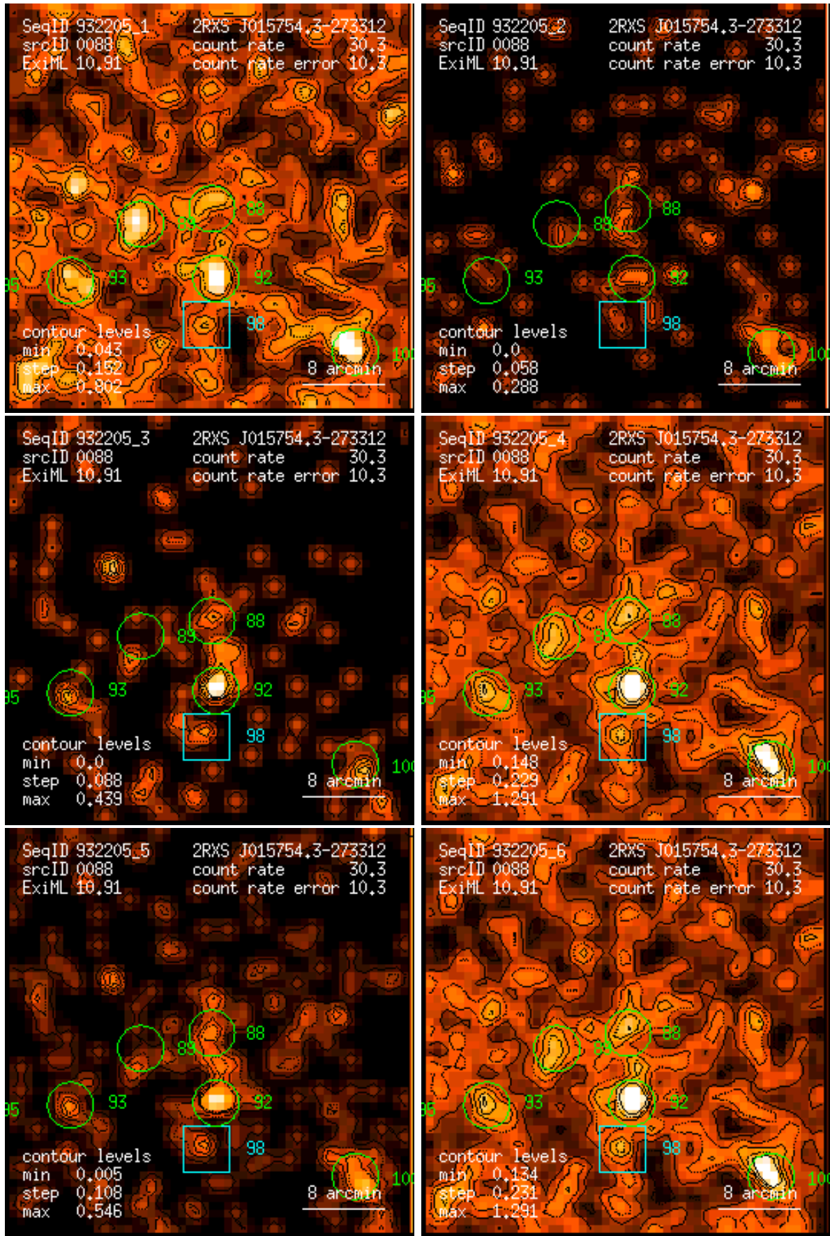
Figure 88: RASS 932205: detection 0088: band rate images, Gaussian filter: (1) PSPC channels 11 – 41, (2) 52 – 90, (3) 91 – 201, (4) 11 – 235, (5) 52 – 201, (6) 11 – 201. Broad band rates in counts/ks. Band rate contour levels in counts/ks/arcmin 2 .
