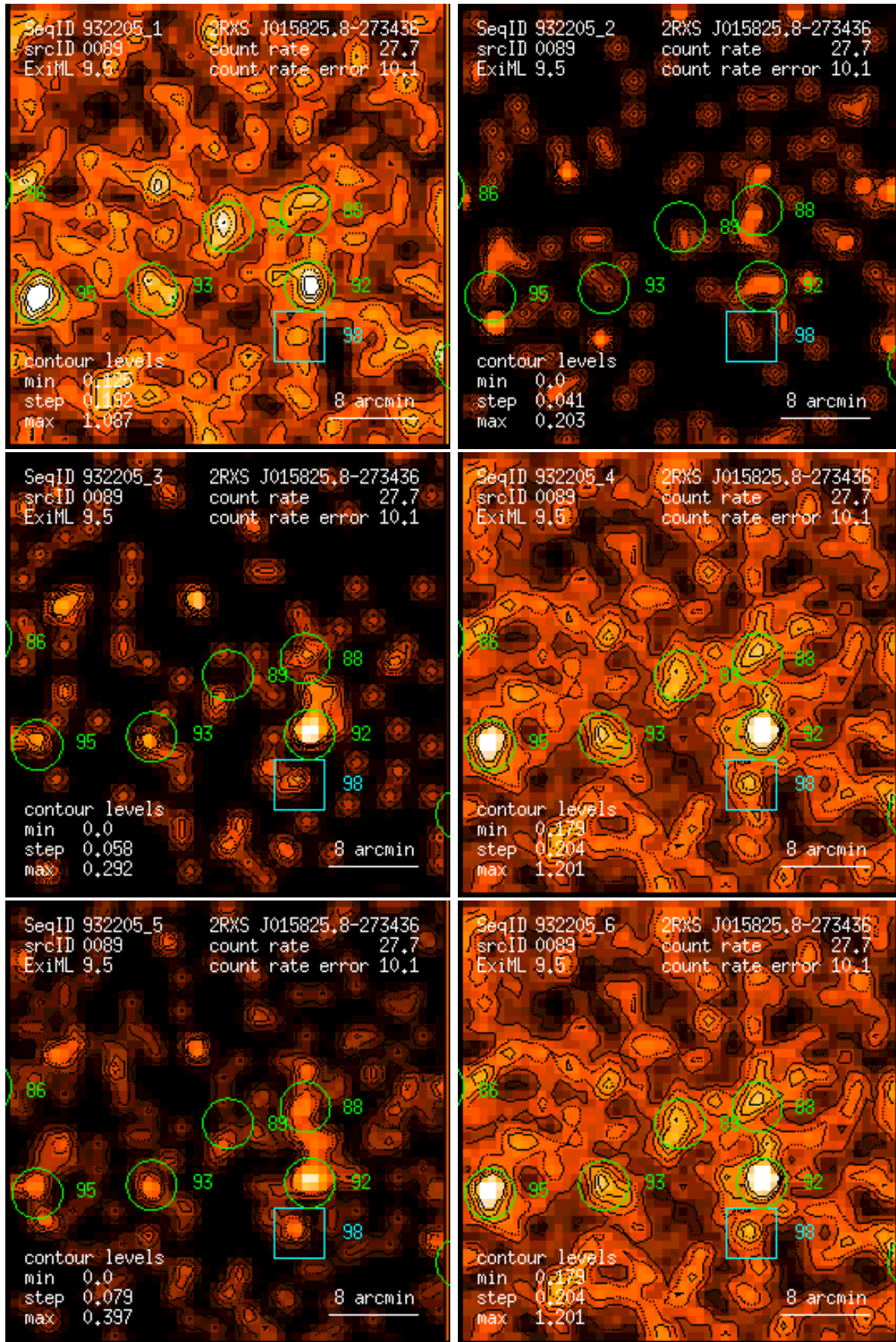
Figure 89: RASS 932205: detection 0089: band rate images, Gaussian filter: (1) PSPC channels 11 – 41, (2) 52 – 90, (3) 91 – 201, (4) 11 – 235, (5) 52 – 201, (6) 11 – 201. Broad band rates in counts/ks. Band rate contour levels in counts/ks/arcmin 2 .
