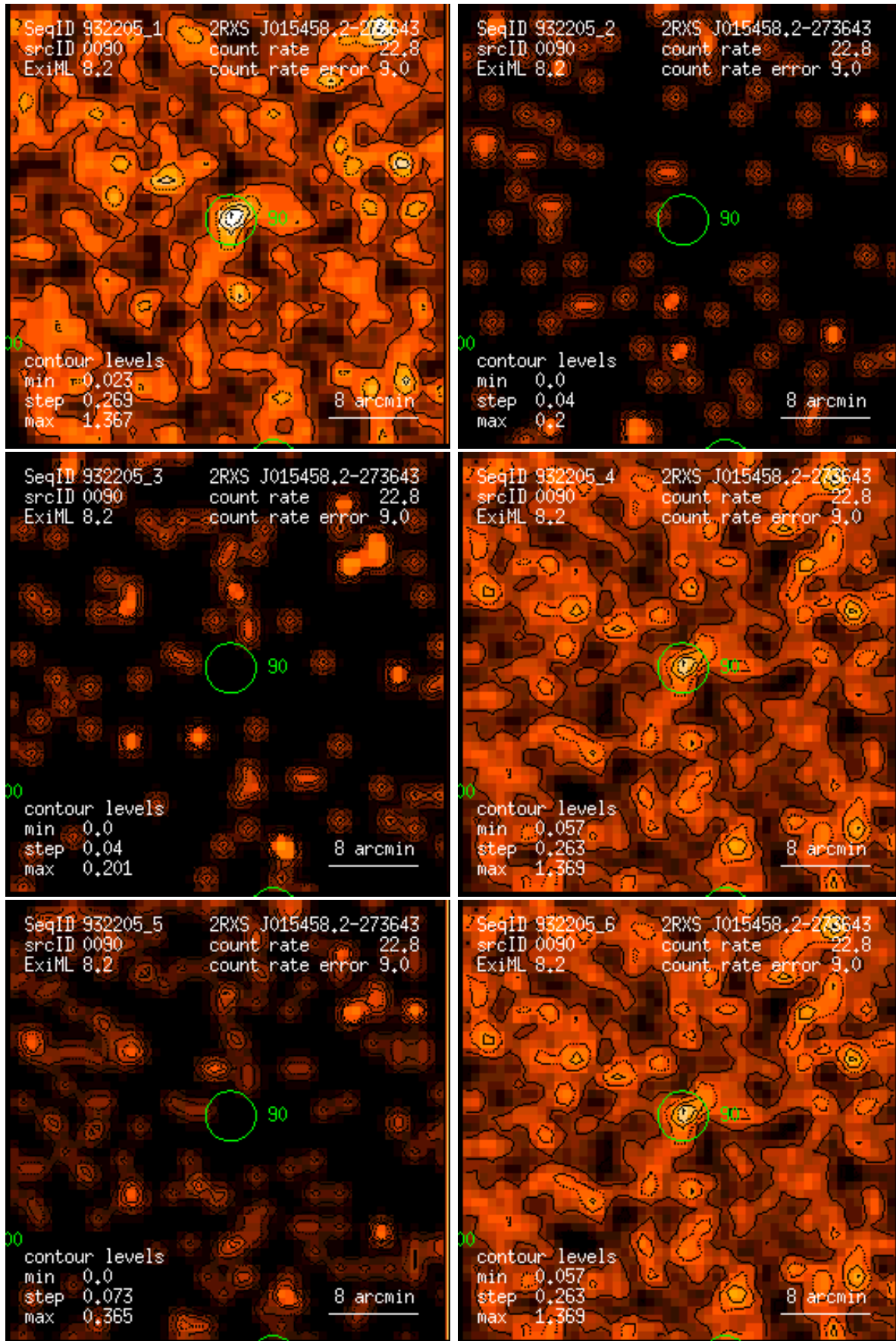
Figure 90: RASS 932205: detection 0090: band rate images, Gaussian filter: (1) PSPC channels 11 – 41, (2) 52 – 90, (3) 91 – 201, (4) 11 – 235, (5) 52 – 201, (6) 11 – 201. Broad band rates in counts/ks. Band rate contour levels in counts/ks/arcmin 2 .
