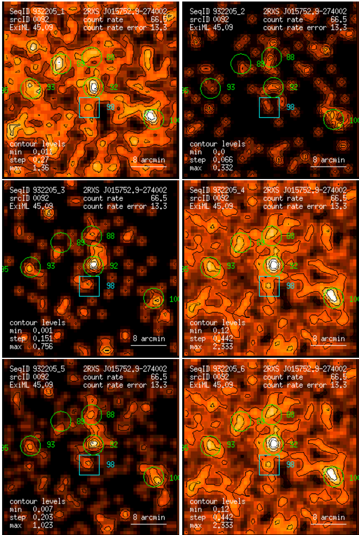
Figure 92: RASS 932205: detection 0092: band rate images, Gaussian filter: (1) PSPC channels 11 – 41, (2) 52 – 90, (3) 91 – 201, (4) 11 – 235, (5) 52 – 201, (6) 11 – 201. Broad band rates in counts/ks. Band rate contour levels in counts/ks/arcmin 2 .
