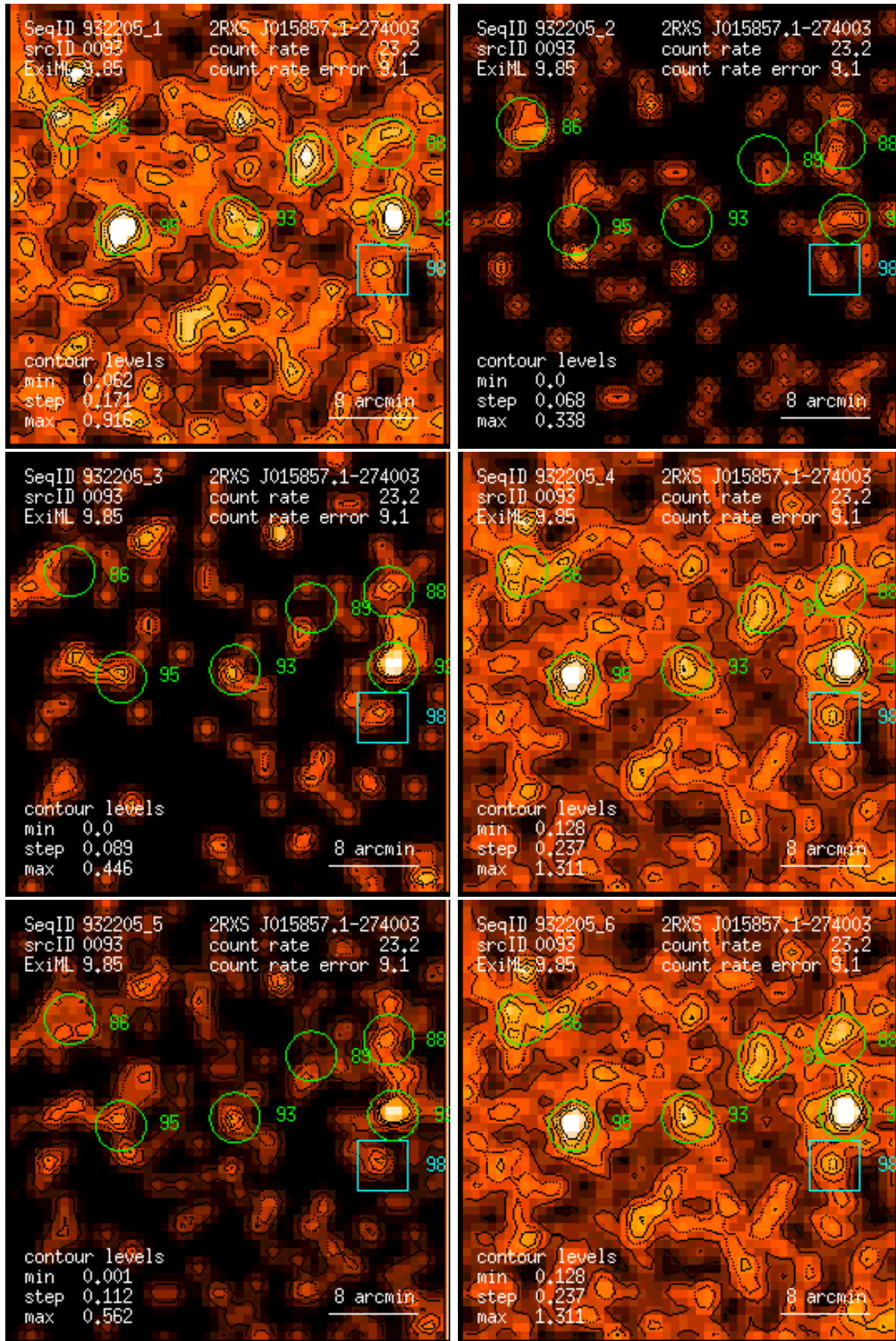
Figure 93: RASS 932205: detection 0093: band rate images, Gaussian filter: (1) PSPC channels 11 – 41, (2) 52 – 90, (3) 91 – 201, (4) 11 – 235, (5) 52 – 201, (6) 11 – 201. Broad band rates in counts/ks. Band rate contour levels in counts/ks/arcmin 2 .
