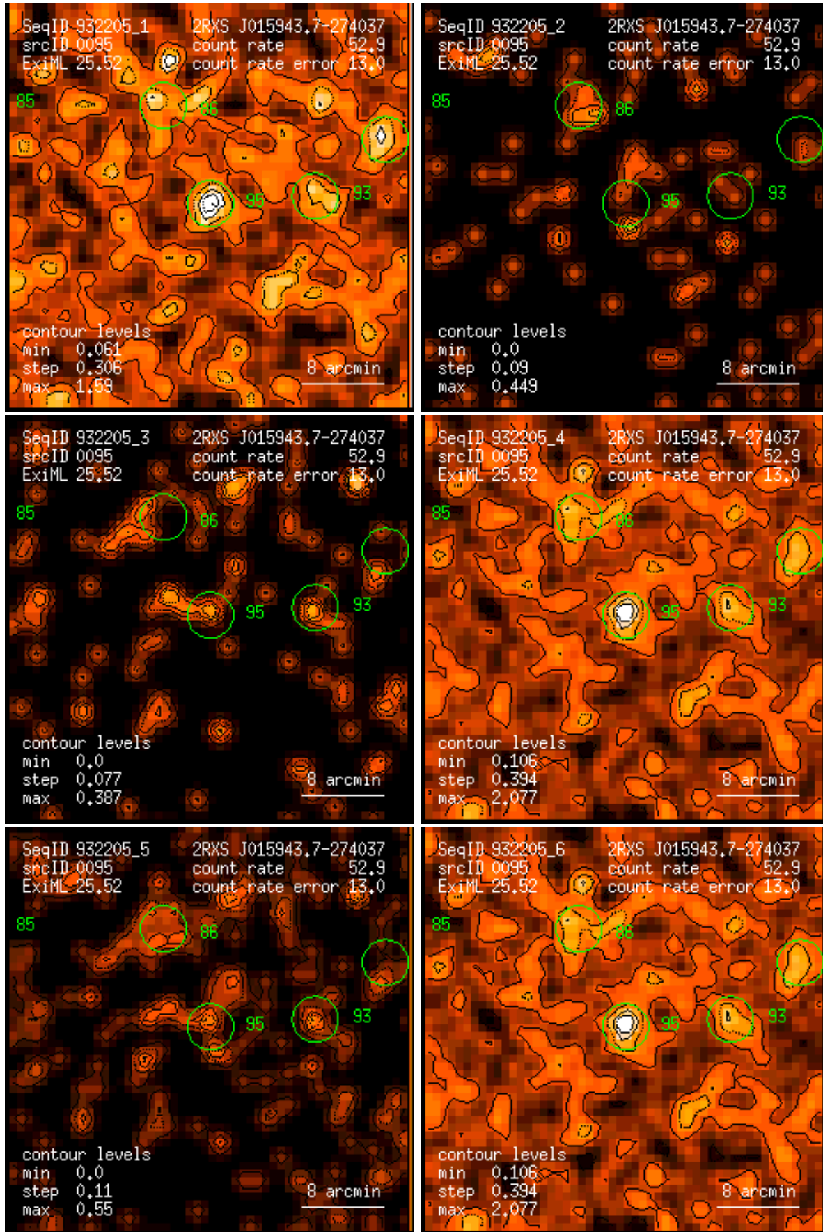
Figure 95: RASS 932205: detection 0095: band rate images, Gaussian filter: (1) PSPC channels 11 – 41, (2) 52 – 90, (3) 91 – 201, (4) 11 – 235, (5) 52 – 201, (6) 11 – 201. Broad band rates in counts/ks. Band rate contour levels in counts/ks/arcmin 2 .
