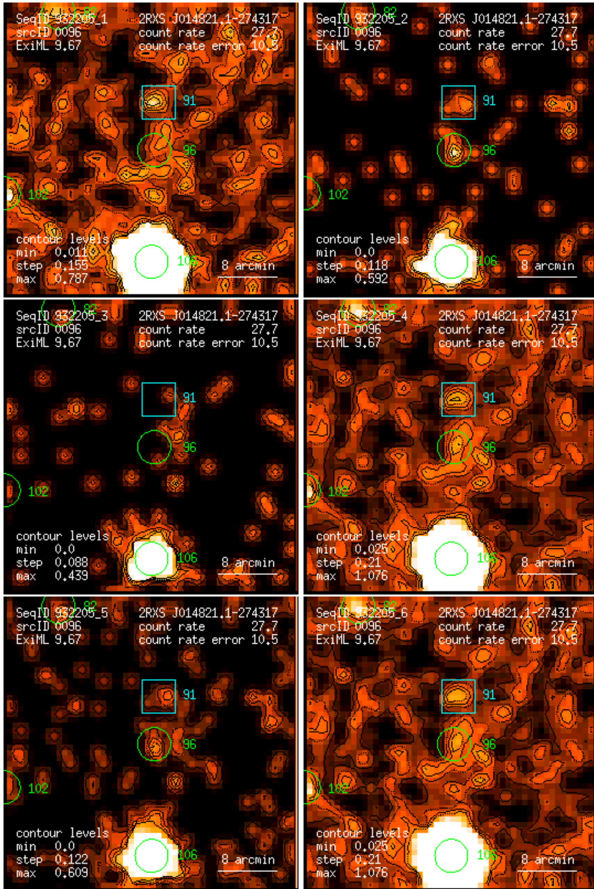
Figure 96: RASS 932205: detection 0096: band rate images, Gaussian filter: (1) PSPC channels 11 – 41, (2) 52 – 90, (3) 91 – 201, (4) 11 – 235, (5) 52 – 201, (6) 11 – 201. Broad band rates in counts/ks. Band rate contour levels in counts/ks/arcmin 2 .
