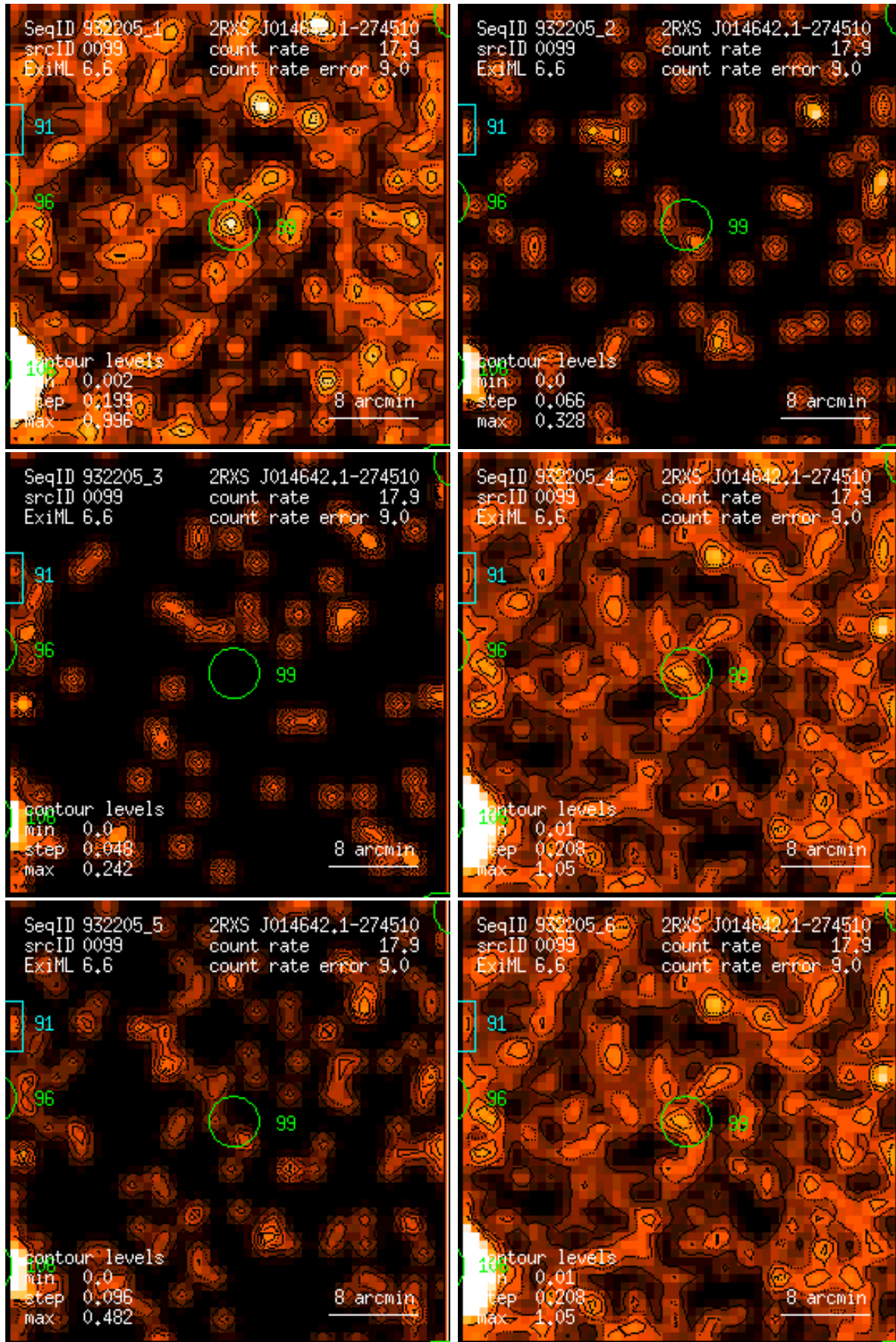
Figure 99: RASS 932205: detection 0099: band rate images, Gaussian filter: (1) PSPC channels 11 – 41, (2) 52 – 90, (3) 91 – 201, (4) 11 – 235, (5) 52 – 201, (6) 11 – 201. Broad band rates in counts/ks. Band rate contour levels in counts/ks/arcmin 2 .
