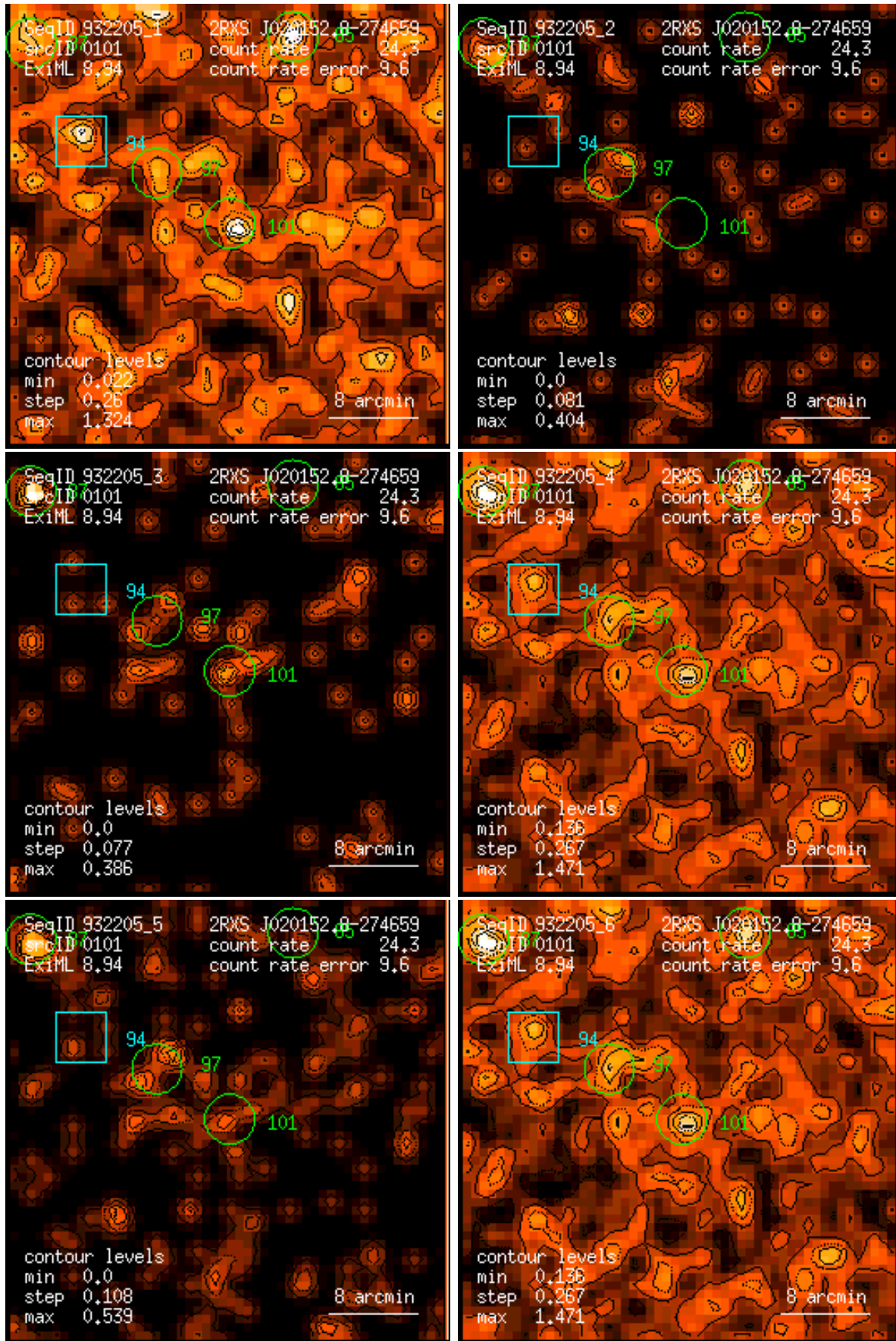
Figure 101: RASS 932205: detection 0101: band rate images, Gaussian filter: (1) PSPC channels 11 – 41, (2) 52 – 90, (3) 91 – 201, (4) 11 – 235, (5) 52 – 201, (6) 11 – 201. Broad band rates in counts/ks. Band rate contour levels in counts/ks/arcmin 2 .
