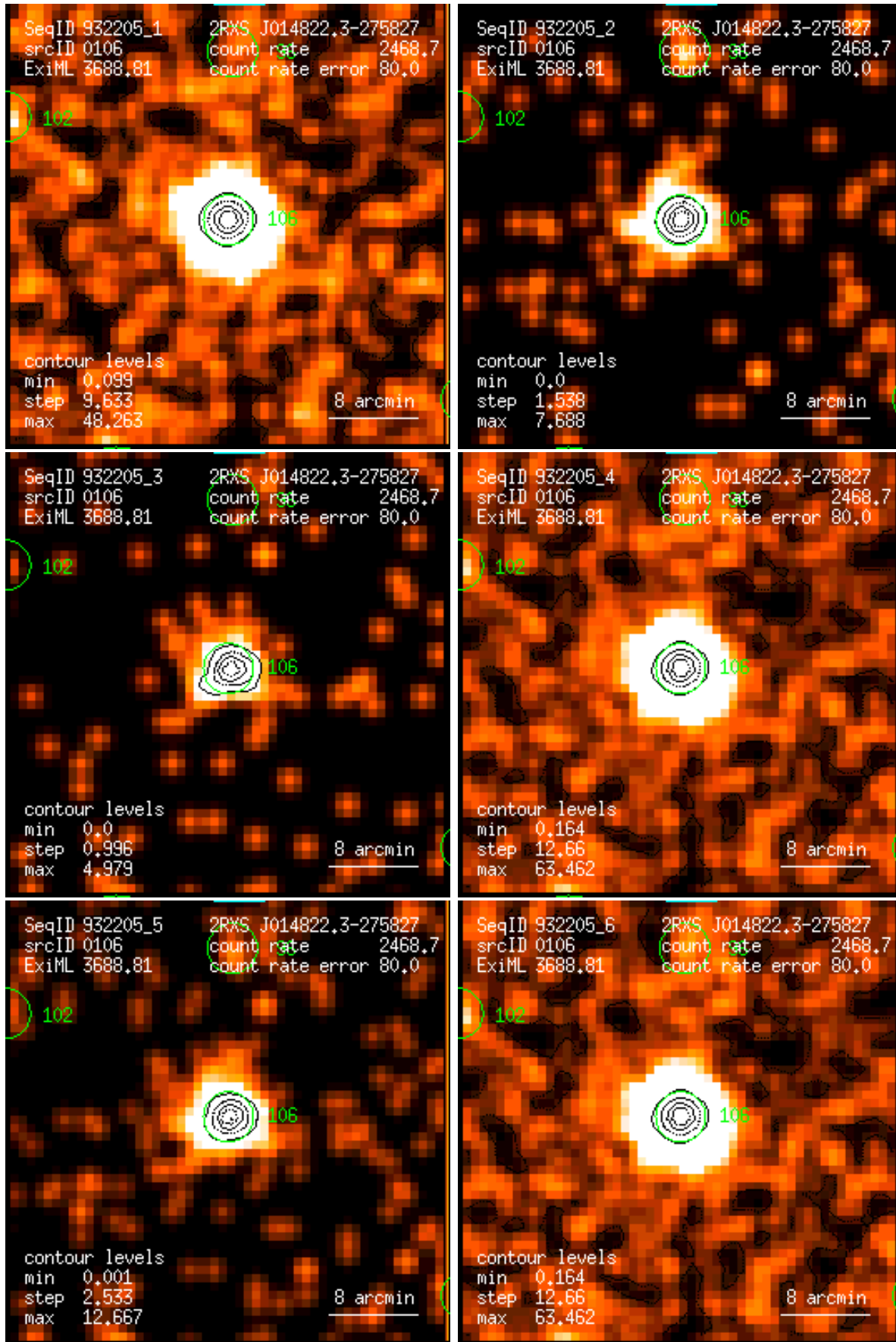
Figure 106: RASS 932205: detection 0106: band rate images, Gaussian filter: (1) PSPC channels 11 – 41, (2) 52 – 90, (3) 91 – 201, (4) 11 – 235, (5) 52 – 201, (6) 11 – 201. Broad band rates in counts/ks. Band rate contour levels in counts/ks/arcmin 2 .
